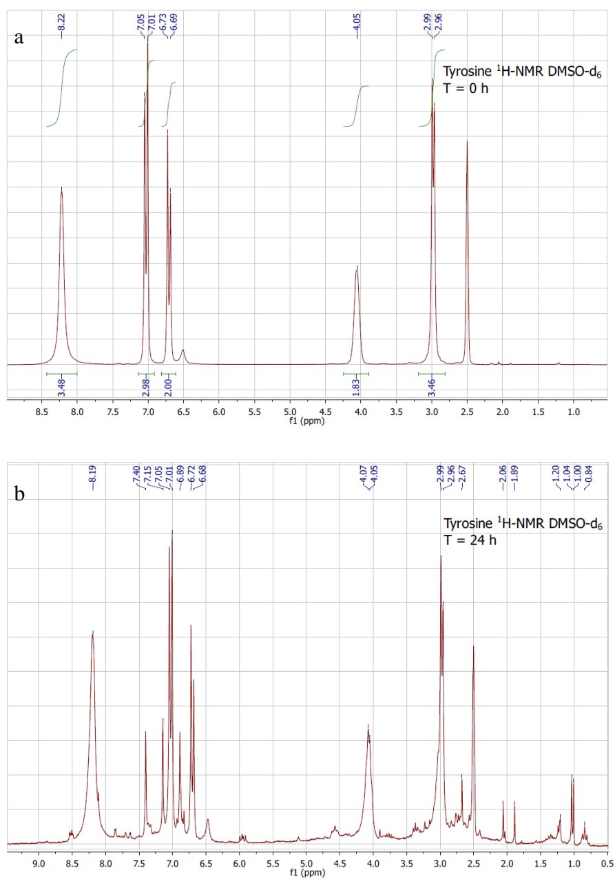
Figure 3. ^1\text{H-NMR} spectra of acidified L-tyrosine before (a) and after 24 h of irradiation (b) ( \text{DMSO-d}_6 ). ^1\text{H NMR} (200 MHz, \text{DMSO-d}_6 ): \delta 8.20 (1H, s, \text{HOPh} ), 7.03 (2H, d, J 8.1 Hz, \text{CHPh} ), 6.71 (2H, d, J 8.1 Hz, \text{CHPh} ), 4.07 (1H, m, \text{CH}_2\text{-CH} ), 2.98 (2H, d, J 6.0 Hz \text{CH}_2\text{-CH} ).
