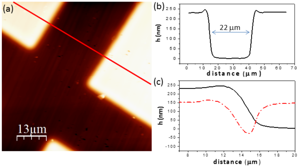
Fig. 2: a) Topography as measured by AFM of a diamond single-crystal sample after irradiation with a 10 MeV Au beam at a fluence of 5 \times 10^{14} \text{ cm}^{-2} . An 80 \mu\text{m} -mesh mask with 60 \mu\text{m} square apertures was used during irradiation. b) Profile along the segment indicated in the image in (a). c) Magnification of the step edge profile (black line) and its derivative (red dot-dashed line) to better visualize the abruptness of the step.
