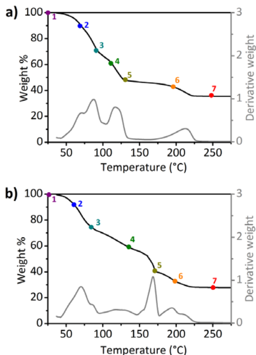
Figure 1. Thermogravimetric (black line) and differential thermogravimetric (grey line) analysis of \text{MgCl}_2\text{-6MeOH} (part a) and \text{MgCl}_2\text{-6EtOH} (part b) under
