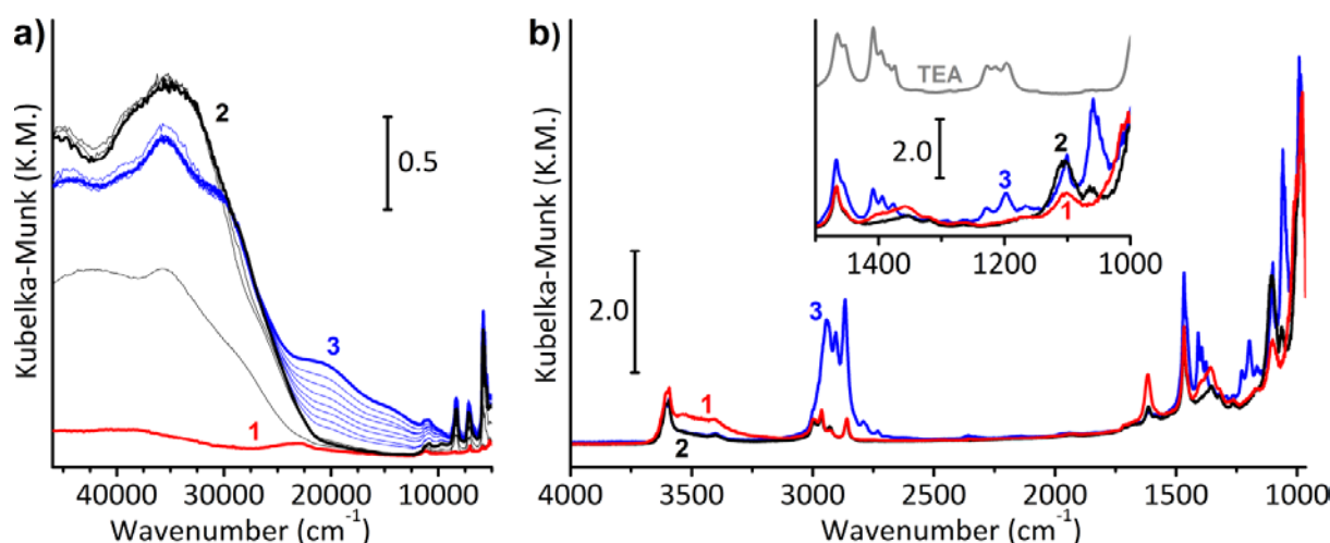
Figure 5. Evolution of the operando diffuse reflectance (DR) UV-Vis-NIR (Part a) and diffuse reflectance infrared Fourier transform (DRIFT) (Part b) spectra upon titration of \text{MgCl}_2\cdot 250 at 90\text{ }^\circ\text{C} with injections of hexane-diluted \text{TiCl}_4 in \text{N}_2 flux (from spectrum 1 to spectrum 2), and upon activation of \text{MgCl}_2\cdot 250/\text{TiCl}_4\cdot 90 at 25\text{ }^\circ\text{C} with injections of hexane-diluted TEA in \text{N}_2 flux (from spectrum 2 to spectrum 3). Inset of part b shows a magnification of the DRIFT spectra in the 1500\text{-}1000\text{ cm}^{-1} region; the spectra are compared with the spectrum of liquid triethylaluminum (TEA) collected in attenuated total reflectance (ATR) mode.
