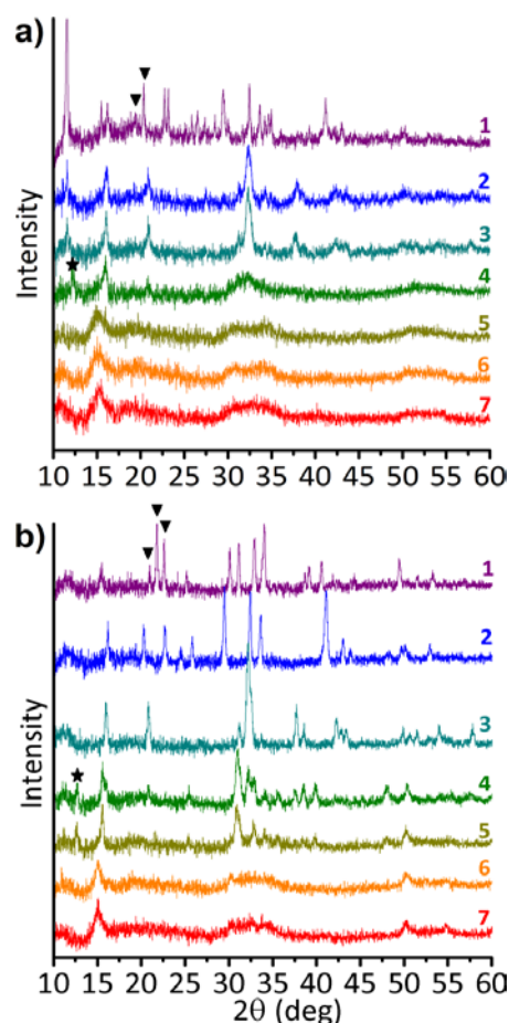
Figure 2. Evolution of the X-ray powder diffraction (XRPD) patterns upon dealcoholation of \text{MgCl}_2\text{-6MeOH} (part a) and \text{MgCl}_2\text{-EtOH} (part b), under \text{N}_2 flux (20 mL/min) at increasing temperatures (2 °C/min), from 25 to 250 °C. The
