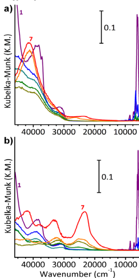
Figure 3. Evolution of the diffuse reflectance (DR) UV-Vis spectra upon dealcoholation of MgCl 2 -6MeOH (part a) and MgCl 2 -EtOH (part b), under N 2 flux (20 mL/min) at increasing temperatures (2 °C/min), from 25 to 250 °C. The color code is the same as in Figure 1 (25, 60, 90, 120, 150, 200 and 250 °C for MgCl 2 -MeOH, and 25, 50, 80, 120, 170, 200 and 250 °C for MgCl 2 -EtOH).
