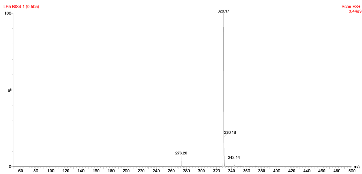
Figure S4. MS spectrum of compound II
