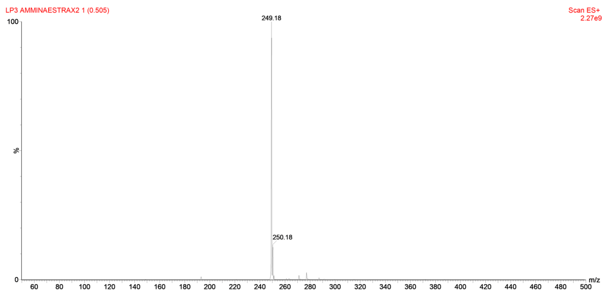
Figure S1: MS spectrum of compound I
