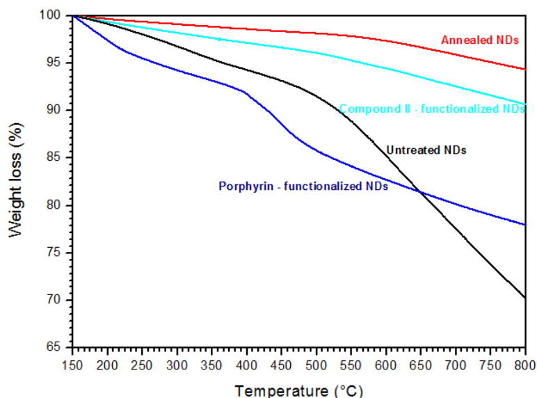
Figure 3 – Thermogravimetric analysis of untreated (black), annealed (red), compound II functionalized (cyan) and porphyrin-functionalized (blue) NDs.
