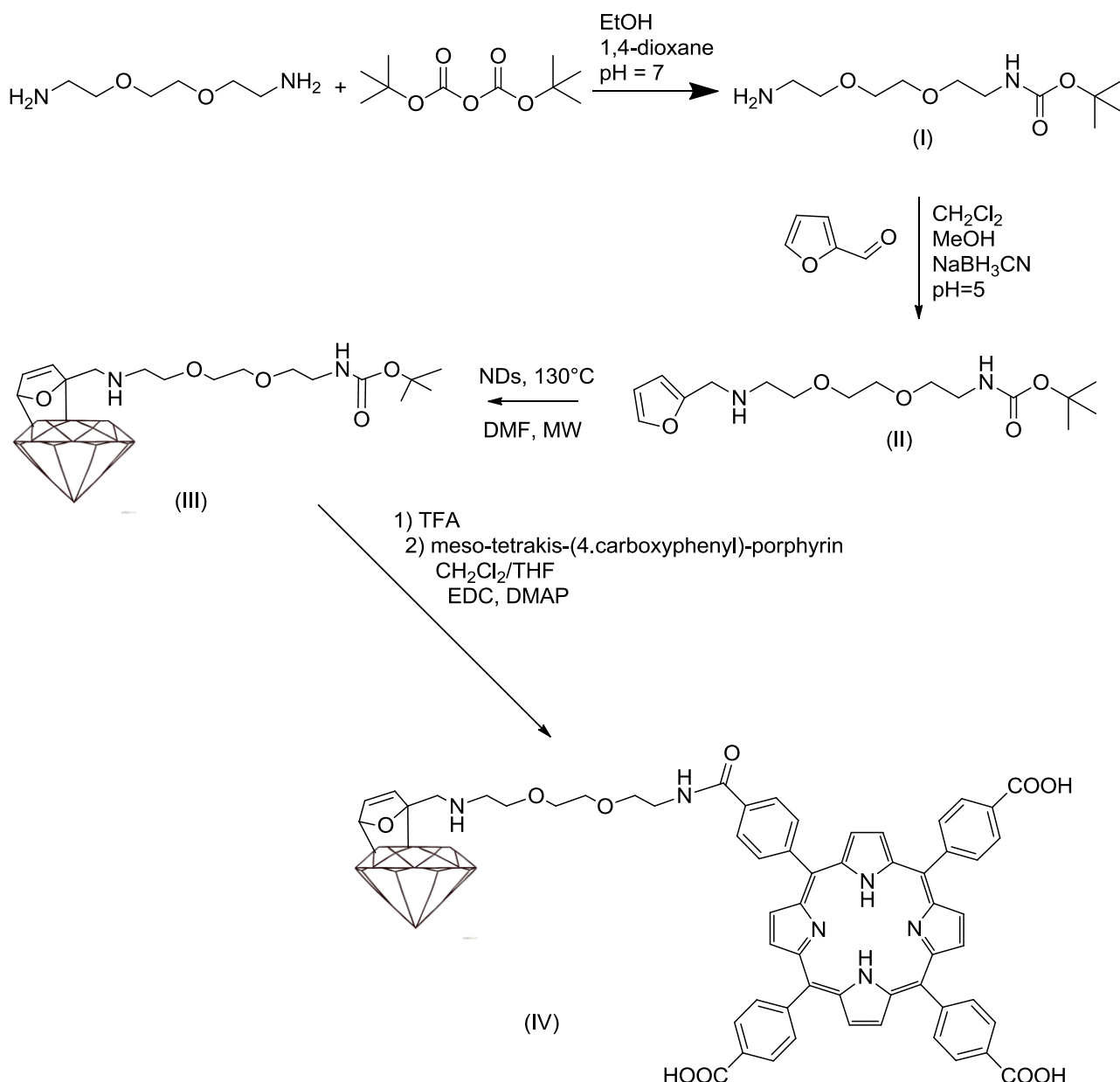
Figure 1 - Synthetic pathway to obtain hybrid nanodiamonds
