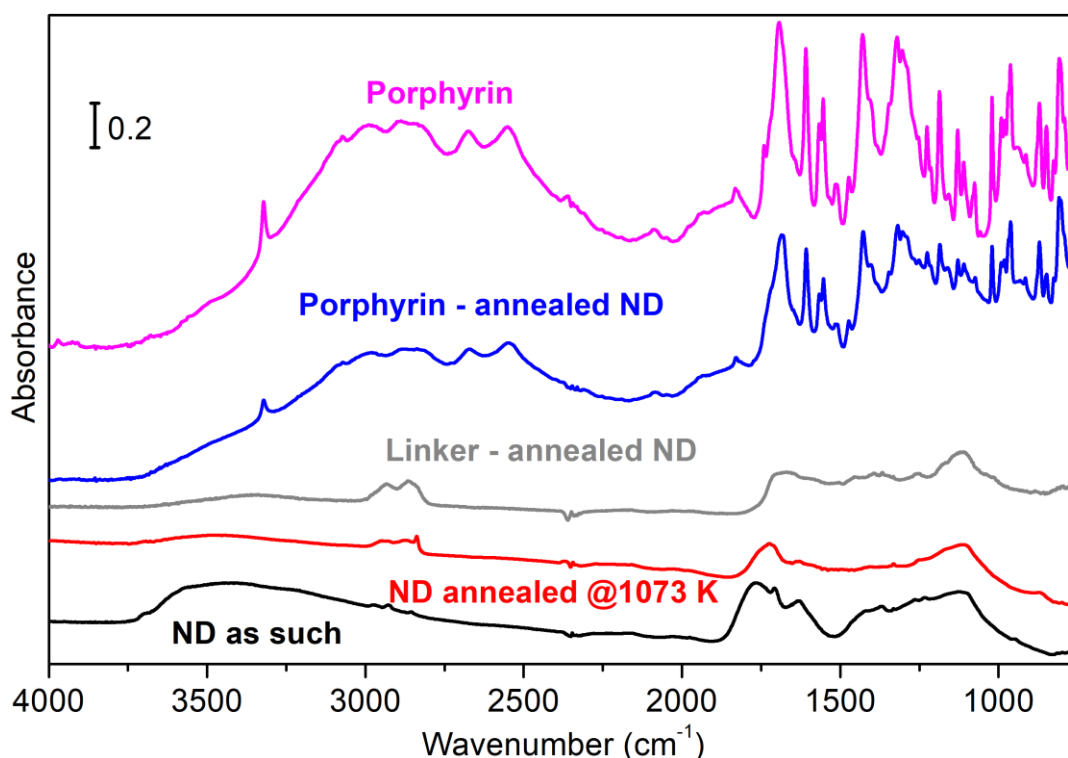
Figure 7 - FT-IR spectra of untreated (black), annealed (red) compound II-functionalized (grey) and porphyrin-functionalized (blue) NDs. The porphyrin spectrum (magenta) is also reported for reference. A magnification of untreated and annealed NDs spectra is available in the figure S7 of supporting information.
