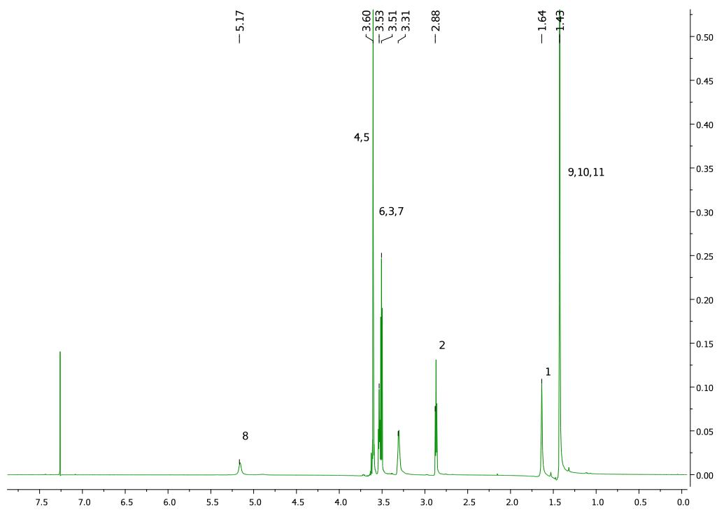
Figure S2. 1 H-NMR spectrum of compound I
