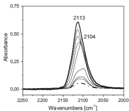
Fig. 12 FTIR spectra collected upon admission of 50 mbar \text{O}_2 at -180 °C over Au/Cu-Mn 2:1 after outgassing (bold line) and under outgassing at increasing temperature (fine lines) up to RT (bold dashed dotted line)
