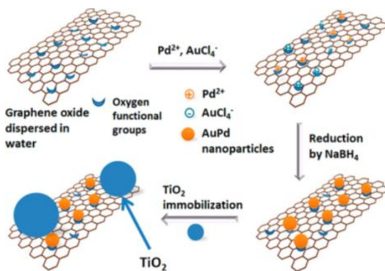
Scheme 5. Illustration of the Method Used for Preparing GO Stabilized Au–Pd nanoparticles on \text{TiO}_2 ( \text{Au-Pd-GO/TiO}_2 ) Using a “Ligand-free” Sol-Immobilization-Type Approach. Reproduced with permission from reference 363 Copyright 2015, ACS.
