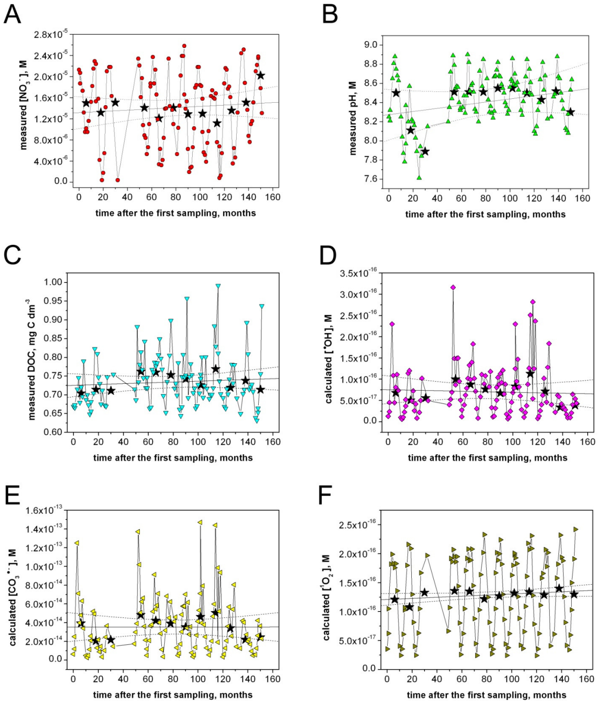
Figure 3. Time trends of \text{NO}_3^- (A), pH (B), DOC (C) and of the modelled steady-state concentration of \cdot\text{OH} (D), \text{CO}_3^{\cdot-} (E) and ^1\text{O}_2 (F) for Lake Garda. The black stars represent the year averages of each relevant parameter, based on which the regression lines (solid) and the 95% confidence bounds (dashed) were calculated.
