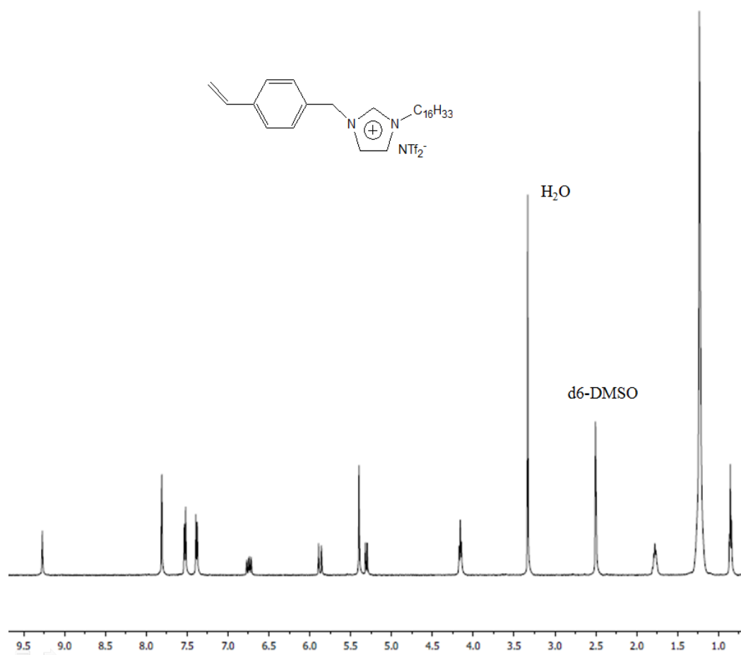
Figure S3. 1 H NMR (Bruker DRX-500 MHz, d 6 -DMSO) spectrum of [VBHDIM][NTf 2 ]: 9.25 (s, 1H), 8.22 (s, 2H), 7.78 (d, 2H), 7.51 (d, 2H), 7.36 (d, 2H), 6.72 (m, 1H), 5.86 (d, 1H), 5.41 (d, 2H), 5.28 (m, 1H), 4.12 (t, 2H), 1.77 (t, 2H), 1.22 (m, 26H), 0.84 (t, 3H).
