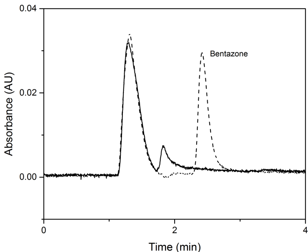
Figure 7. Chromatograms of the solution before the treatment (dashed line) and collected at the outlet of the fourth column (continuous line).
