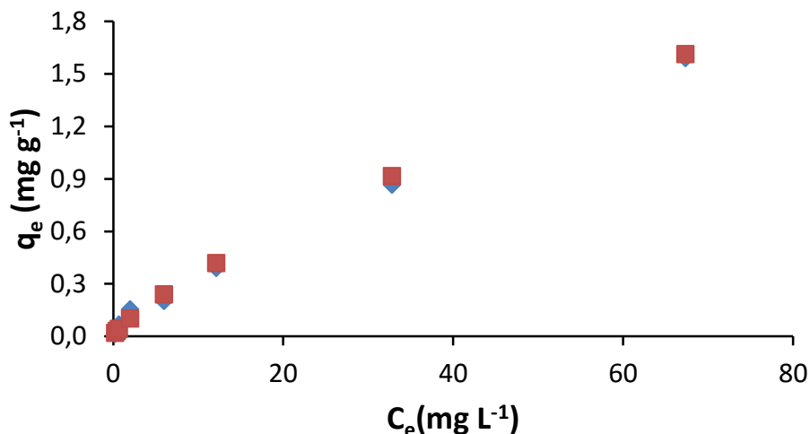
Figure 4. Adsorption isotherm for bentazone onto MS1. Experimental (▼) and calculated (■) values according to linearized Freundlich model. Experimental conditions: 0.2 g of MS1 in contact with 10 mL of bentazone solutions (pH 2.5, range 0.5-100 mg L -1 ), stirred at room temperature for 26 h.
