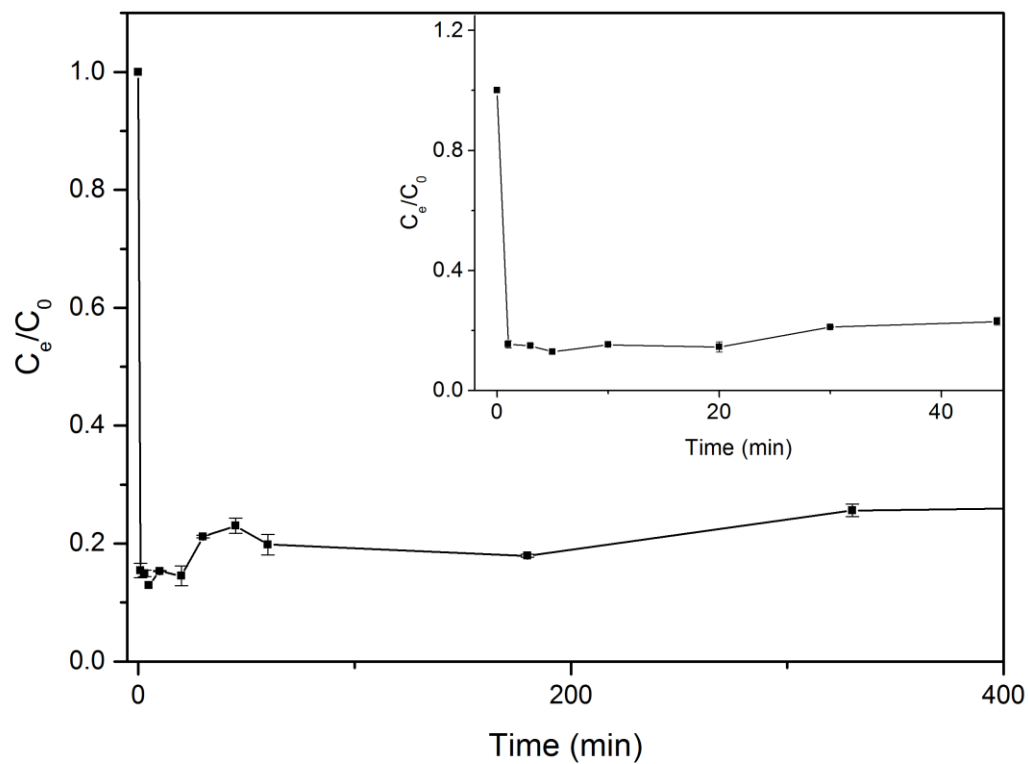
Figure 2: Bentazone adsorption ( 2 \text{ mg L}^{-1} , 50 \text{ mL} , \text{pH } 2.5 ) on 1 \text{ g MS1} as a function of contact-time.
