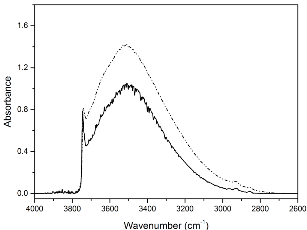
Figure 3: FT-IR spectra of MS1 before (continuous line) and after (dotted line) contact with bentazone solution.
