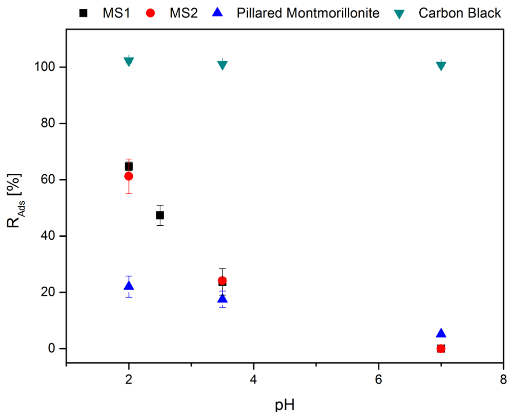
Figure 5. Comparison of bentazone adsorption on different substrates (0.2 g each) at different pH values. Bentazone concentration: 2 mg L -1 (10 mL), contact-time 66 h. Error bars are also shown.
