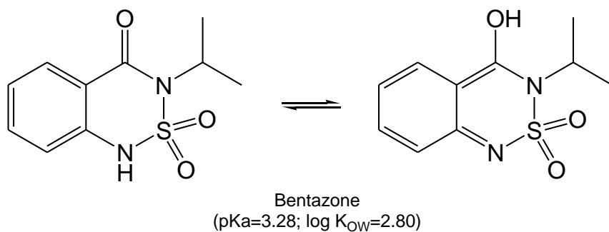
Figure 1. Keto-enol tautomerism of bentazone
