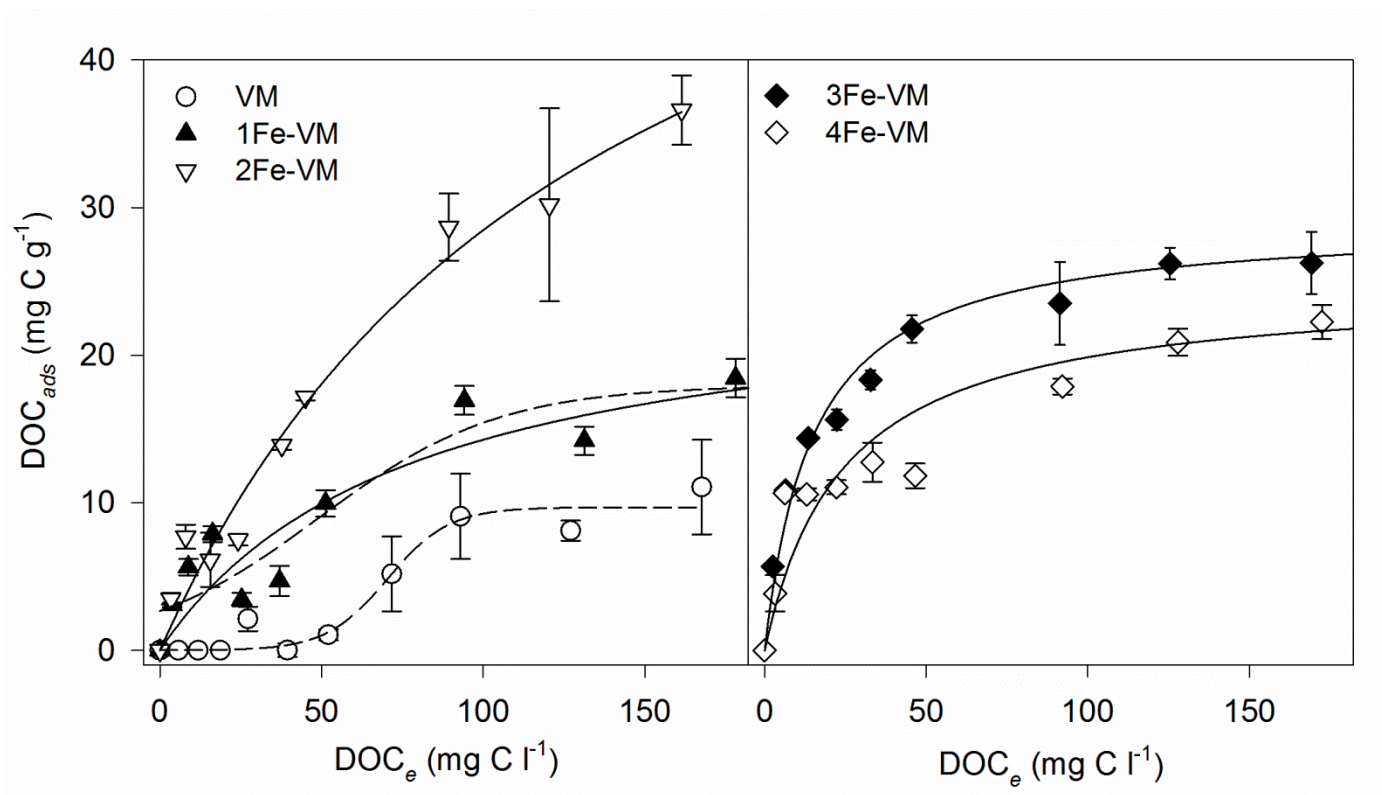
Figure 4: Sorption isotherms of DOC on vermiculite (VM) and Fe (hydr)oxide-vermiculite systems ( x\text{Fe-VM} ) at pH 5.5. Experimental data (symbols) were modelled with the Langmuir (complete line) and sigmoidal (dashed lines) equations. Error bars represent the standard error of the mean.
