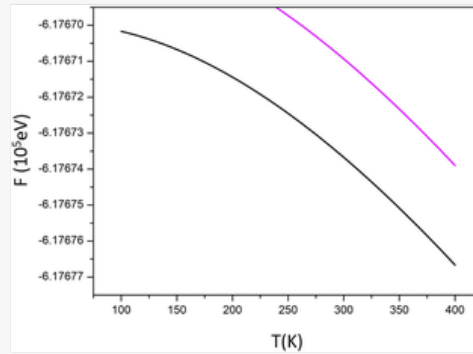
Helmholtz free energy variation with temperature for pseudo-cubic m Model 2 (black line) and monoclinic structure (magenta) of argyrodite at 0 GPa.
