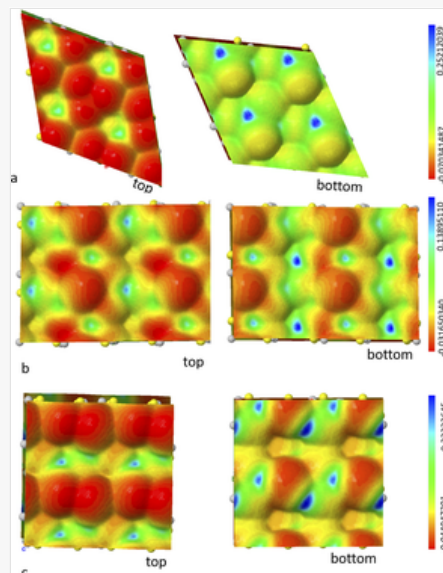
Electrostatic potential (in a.u.) as mapped on an electron charge density isosurface computed at a regular 3-dimensional grid of points for most stable surfaces of model 2: 111 surface (panel a) (mapped on 0.001 \text{ e bohr}^{-3} charge density surface), 110 (panel b, mapped on 0.0003 \text{ e bohr}^{-3} charge density surface), 001 (panel c, mapped on 0.0008 \text{ e bohr}^{-3} charge density surface); both top and bottom views are reported. The blue colour codifies the regions in which the potential is positive while the red colour corresponds to negative values of potential; the green colour represents neutrality.
