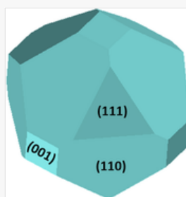
Wulff's polar plot for cubic symmetry of argyrodite based on computed E_S at PBE0/TZVP, the corresponding families of planes are indicated on faces.
