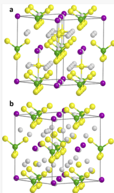
(a) Model 1 with Li introduced in 24g site in cubic space group F43m at PBE0/TZVP. Li atoms are in light gray color, Cl in magenta, P in green, and S in yellow color. (b) Model 2 with Li introduced in 24g site in space group P1 at PBE0/TZVP. Li atoms are in light gray color, Cl in magenta, P in green, and S in yellow color.
