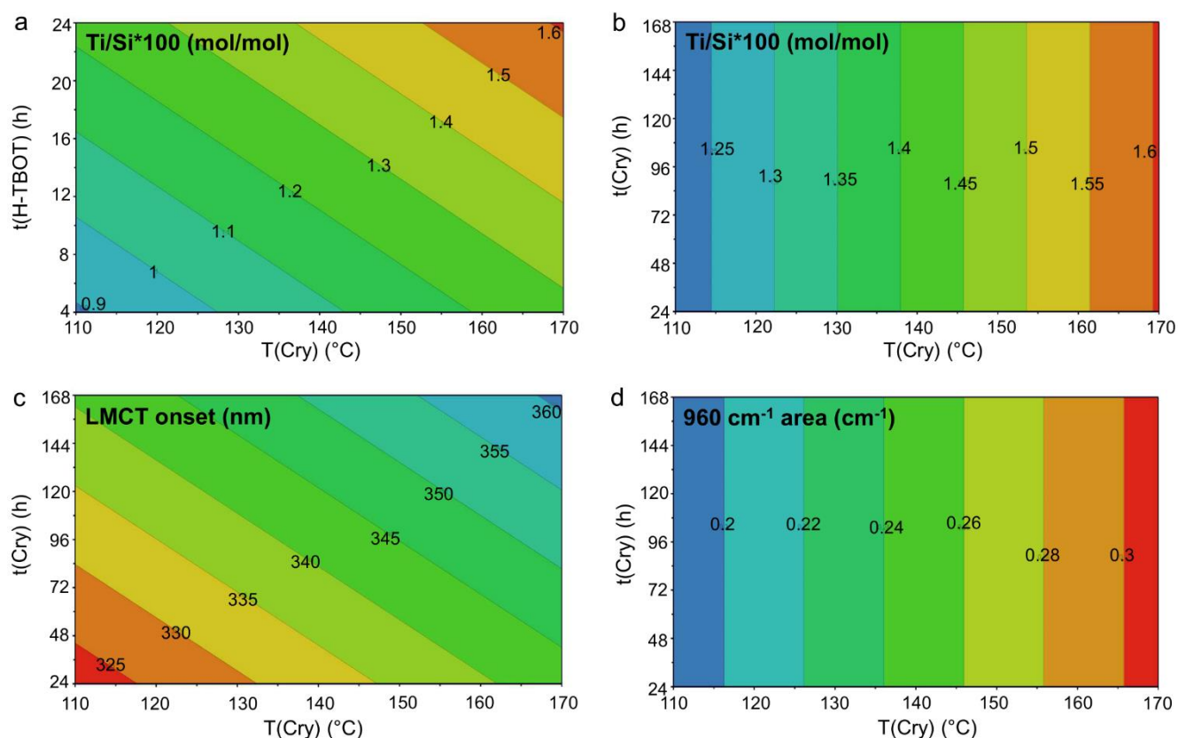
Figure 3. Contour plots for the responses regarding Ti content (Ti/Si*100 in panels a and b) and speciation (LMCT onset in panel c and 960 cm -1 area in panel d). Panels a and c report the contour plots involving the significant variables for the responses Ti/Si*100 and LMCT onset, while panels b is included to compare the total Ti content with the LMCT onset and the 960 cm -1 area varying the same variables (time and temperature of crystallization). The askew bands are iso-response regions, delimited by lines which corresponding response is reported in the labels (the label have the dimension of the response).
