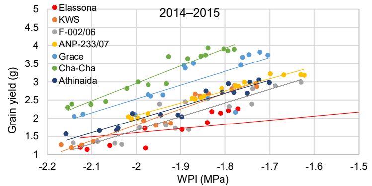
Figure 5. The fitted linear regressions between grain yields (g) per plant and water potential index (WPI) during the first season(left) and second season(right).
