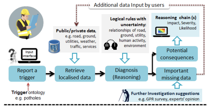
Figure 9: Workflow in the ATU-DSS (from the left to right) (Wei et al., 2018).
