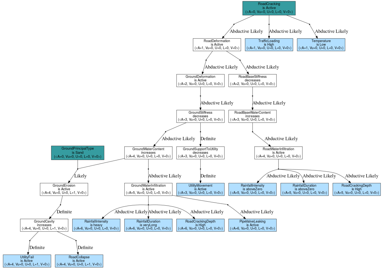
Figure 7: An example of city infrastructure assessment with diagnosis and predictive inference. Colour scheme: turquoise for input facts, white for inferred facts, and light blue for final conclusions.
