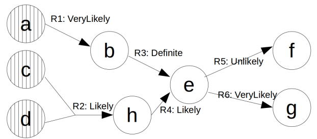
Figure 5: A direct graph representing six predictive rules in a knowledge base (shaded circles for given facts and white circles for derived facts.).
