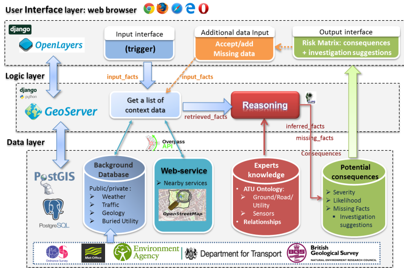
Figure 8: A three-layer system architecture of the ATU-DSS prototype.
