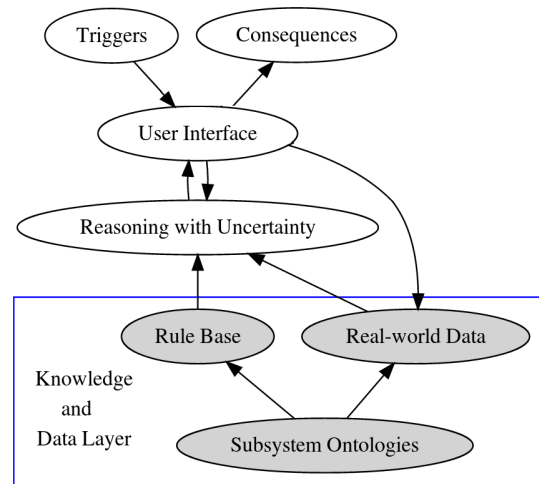
Figure 1: Building blocks of the ATU-DSS: given a trigger, an inference engine is able to predict the potential consequences by reasoning with uncertain data and rules developed based on a set of modular ontologies.
