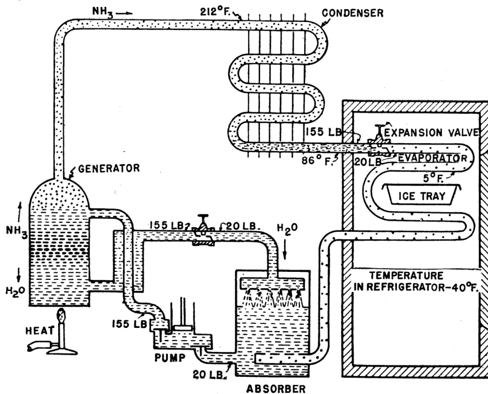
Figure 3.2: Diagrammatic sketch of Ferdinand Carré's absorption refrigeration machine for which he received a patent in the 1860s (Jordan and Priester 1950).
