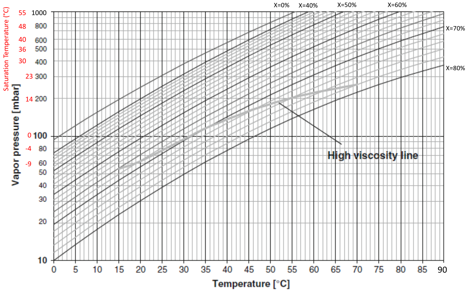
Figure 4.3: Pressure and temperature graph for acetone and zinc bromide solution, where the saturation temperature of pure acetone (red) is next to the corresponding vapour pressure and X is solution concentration in \frac{m_{ZnBr_2}}{m_{solution}} (Ajib and Karno 2008).
