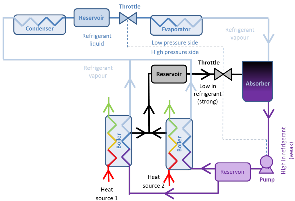
Figure 3.11: Double boiler cycle schematic; showing one absorption refrigerator powered by two discontinuous heat sources through two separate boilers with reservoirs to allow for continuous cooling from discontinuous heat sources.
