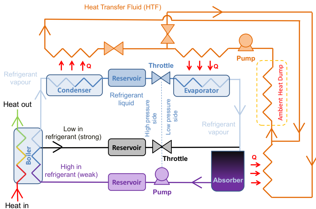
Figure 3.14: Single effect cycle with reservoirs and evaporator tap-off. This cycle allows both continuous refrigeration from discontinuous heat sources and control over the evaporator temperature. The thermal coupling is illustrated as a heat transfer fluid (orange section).
