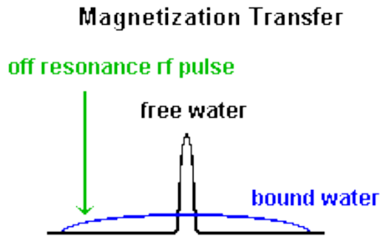
(Figure1.3) Variation in absorption lineshape causing macromolecular selective saturation
