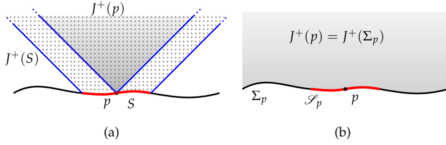
Figure 4: Difference between the notions of causal future in locally Lorentz invariant theories (A) and theories with a preferred foliation (B).
