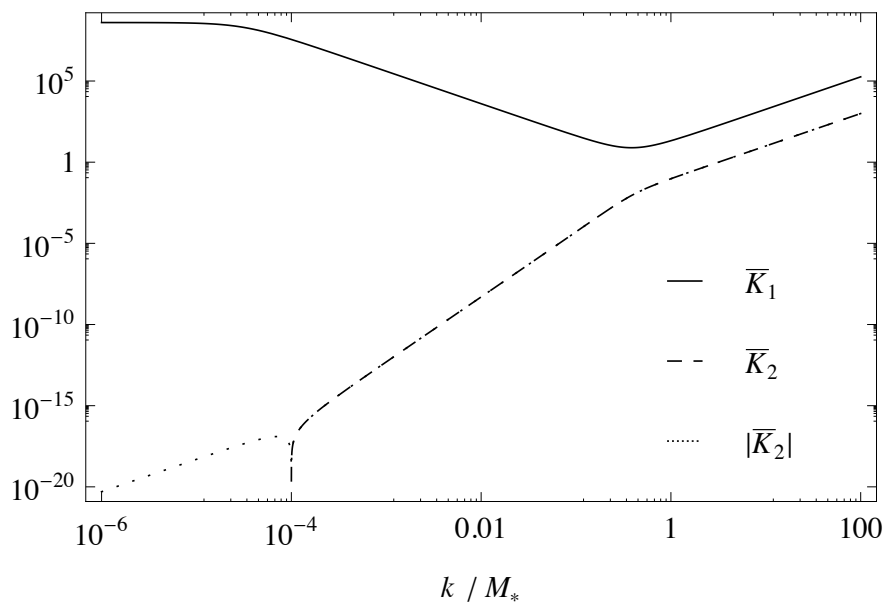
Figure 2: The kinetic matrix eigenvalues (3.59) for the parameter set (3.76). The first eigenvalue (solid line) corresponds to the scalar graviton of Hořava gravity, while the second eigenvalue (dashed line, with absolute value shown as dotted line) corresponds to the new degree arising from the mixed derivative extension. With the chosen parameters, the latter ceases being a ghost at momenta k \simeq 10^{-4}M_* .
