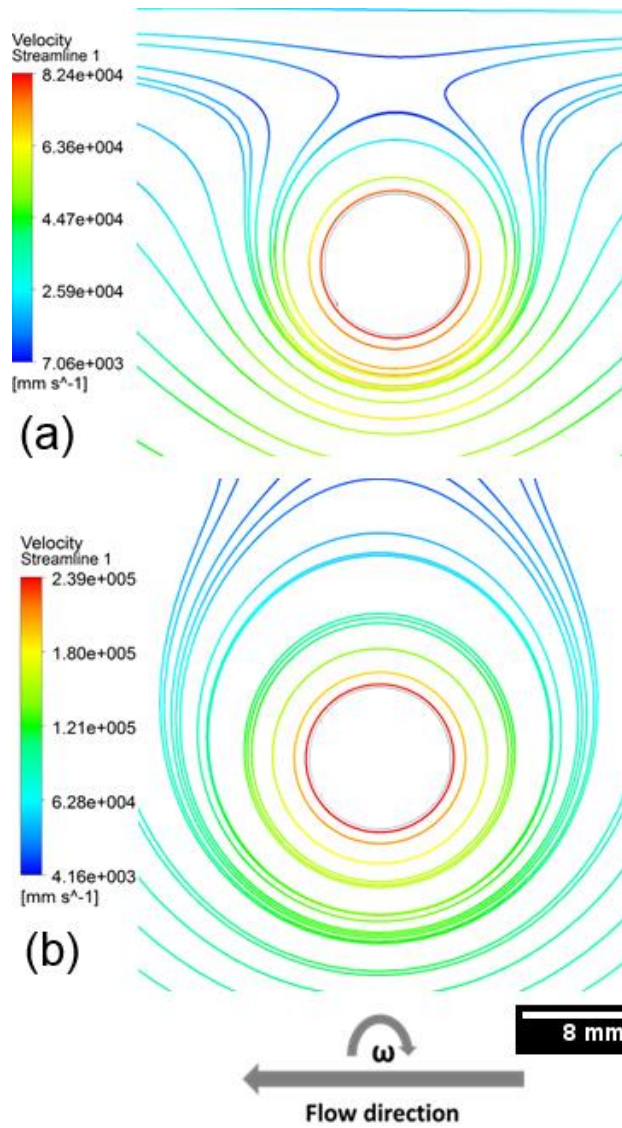
Figure 4-16 (a)- Re = 0.01 \alpha_r = 1 , (b)- \alpha_r = 3 with constant value of viscosity value ( =1.78 \times 10^5 Pa s)
