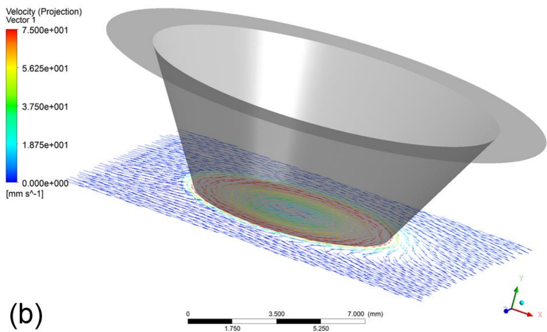
Figure 7-10 Velocity vectors for the conical tool design at 225 rpm and 2.5 \text{ mm s}^{-1} traverse speed for the initial geometry on the plane at the tool tip: (a) in 3D; (b) on the same plane including the tool (shows tool contact with the plane of the velocity vectors).
