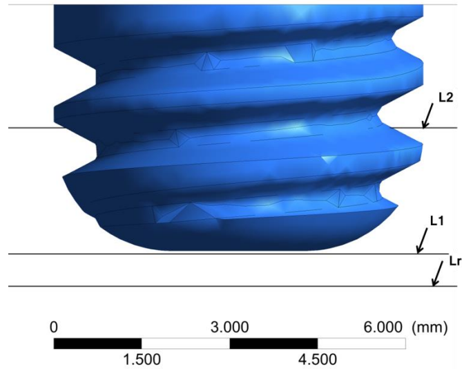
Figure 5-8: Locations used for comparison of MAZ between unworn and worn tool geometries
