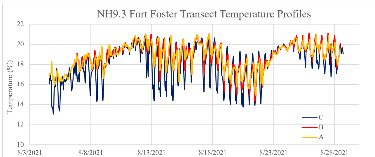
Figure 13. Temperature data collected by HOBO sensors (every 10 minutes) at Transects A, B, and C at site NH9.3 (Fort Foster), 8/4/2021 – 8/28/2021. Note that the vertical axis starts at 10° C.
