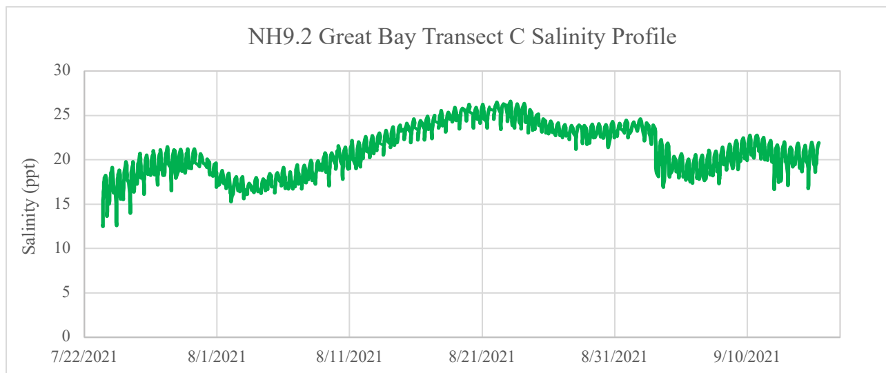
Figure 14. Salinity data collected by a HOBO sensor (every 10 minutes) at Transect C, site NH9.2 (Great Bay), 7/23/2021 – 9/15/2021.
