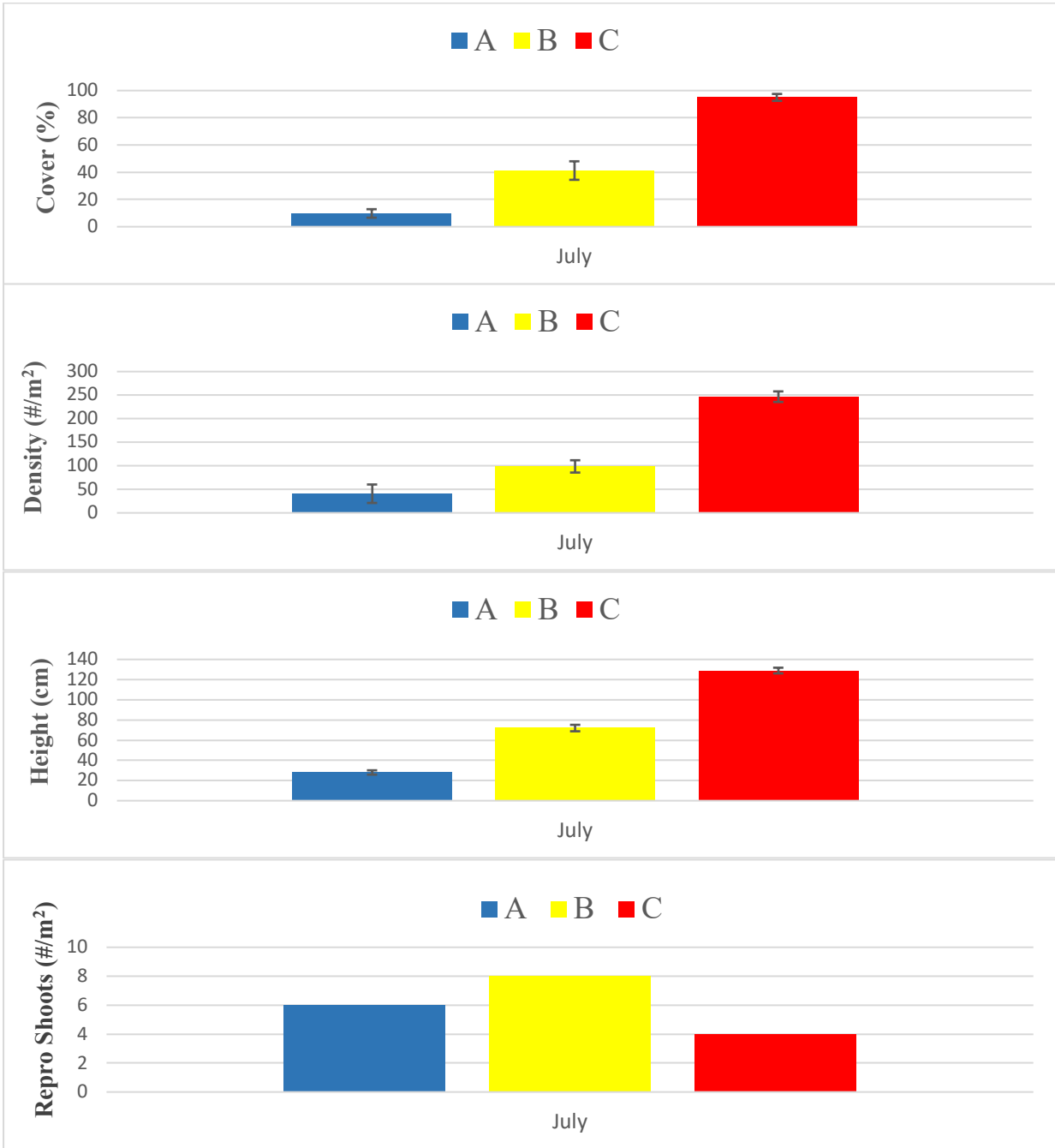
Figure 8. Eelgrass percent cover, shoot density, canopy height, and number of reproductive shoots at SeagrassNet site NH9.2, Transects A, B, and C in Great Bay for 2021. All values are averages except for number of reproductive shoots, which are medians. Error bars indicate Standard Error of the means.
