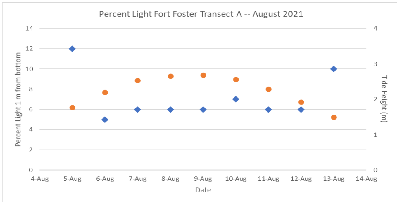
Figure 17. Mean values (blue diamonds) of percent light at 1 m from the bottom at Transect A, site NH9.3 (Fort Foster), 8/5/2021 – 8/13/2021. Values represent means from data collected by HOBO sensors every 10 minutes, between 10 a.m. and 2 p.m. Tide height at noon in meters (orange circles) is plotted on the secondary axis
