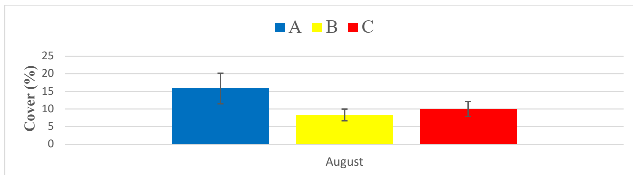
Figure 11. Seaweed percent cover at site NH9.3 (Fort Foster), Transects A, B, and C for August 2021. Error bars indicate Standard Error of the means.
