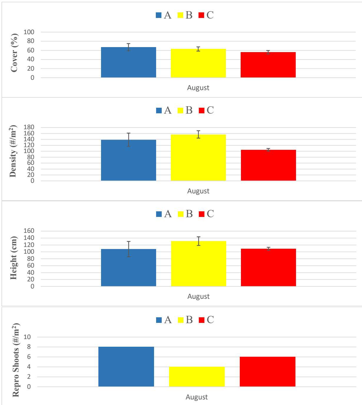
Figure 9. Eelgrass percent cover, shoot density, canopy height, and number of reproductive shoots at SeagrassNet site NH9.3, Transects A, B, and C at Fort Foster for 2021. All values are averages except for number of reproductive shoots, which are medians. Error bars indicate Standard Error of the means.
