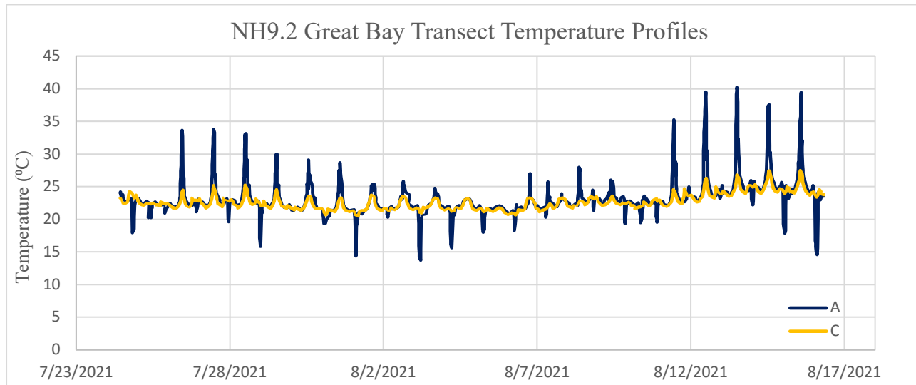
Figure 12. Temperature data collected by HOBO sensors (every 10 minutes) at Transects A and C at site NH9.2 (Great Bay), 7/24/2021 – 8/16/2021.
