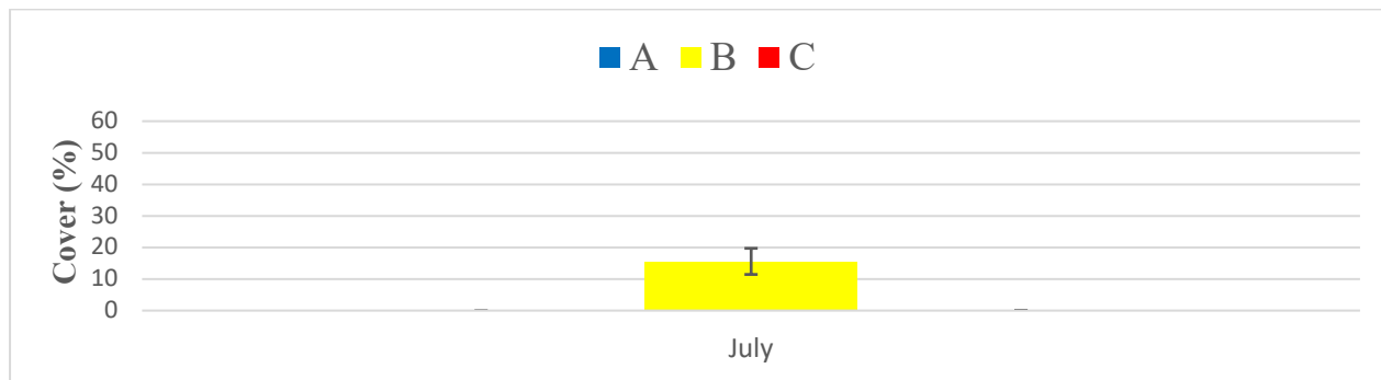
Figure 10. Seaweed percent cover at site NH9.2 (Great Bay), Transects A, B, and C for July 2021. Error bars indicate Standard Error of the means.
