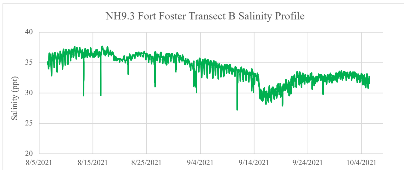
Figure 15. Salinity data collected by a HOBO sensor (every 10 minutes) at Transect B, site NH9.3 (Fort Foster), 8/6/2021 – 10/5/2021. Note that the vertical axis starts at 20 ppt.
