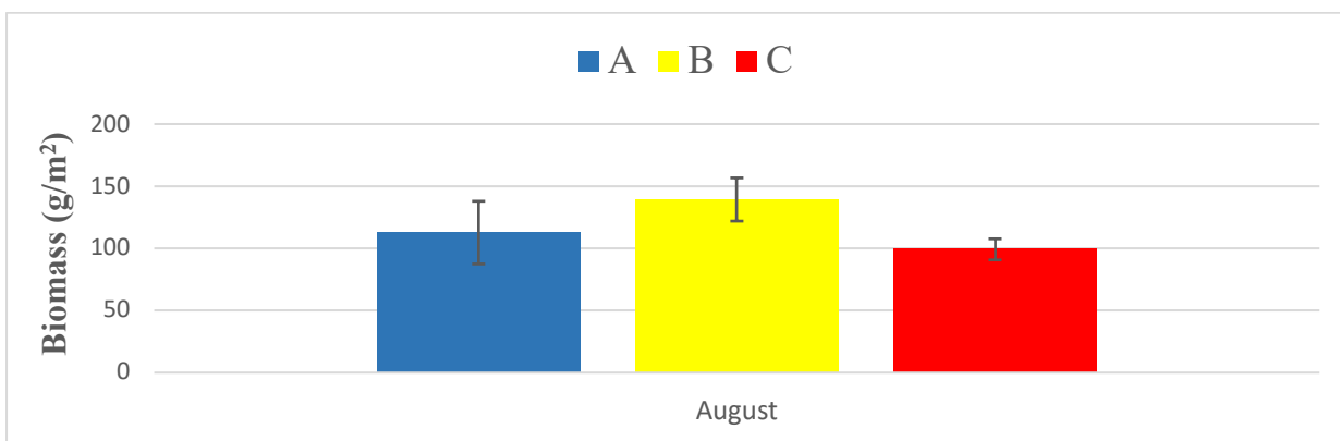
Figure 7. Eelgrass biomass at SeagrassNet site NH9.3 (Fort Foster), Transects A, B, and C for 2021. Error bars indicate Standard Error.
