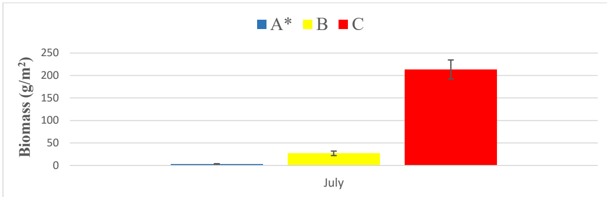
Figure 6. Eelgrass biomass at SeagrassNet site NH9.2 (Great Bay), Transects A, B, and C for 2021. Error bars indicate Standard Error. *60% of Transect A were reproductive plants.
