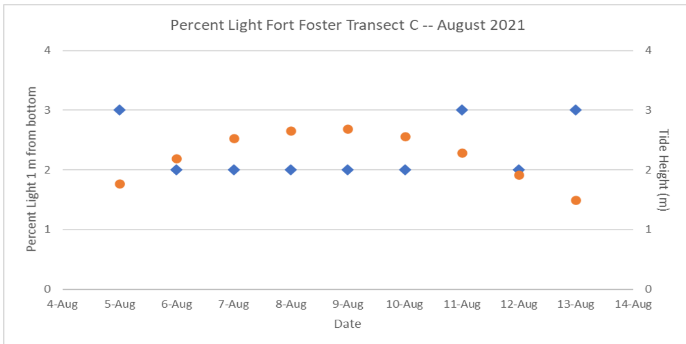
Figure 18. Mean values (blue diamonds) of percent light at 1 m from the bottom at Transect C, site NH9.3 (Fort Foster), 8/5/2021 – 8/13/2021. Values represent means from data collected by HOBO sensors every hour, between 10 a.m. and 2 p.m. Tide height at noon in meters (orange circles) is plotted on the secondary axis.
