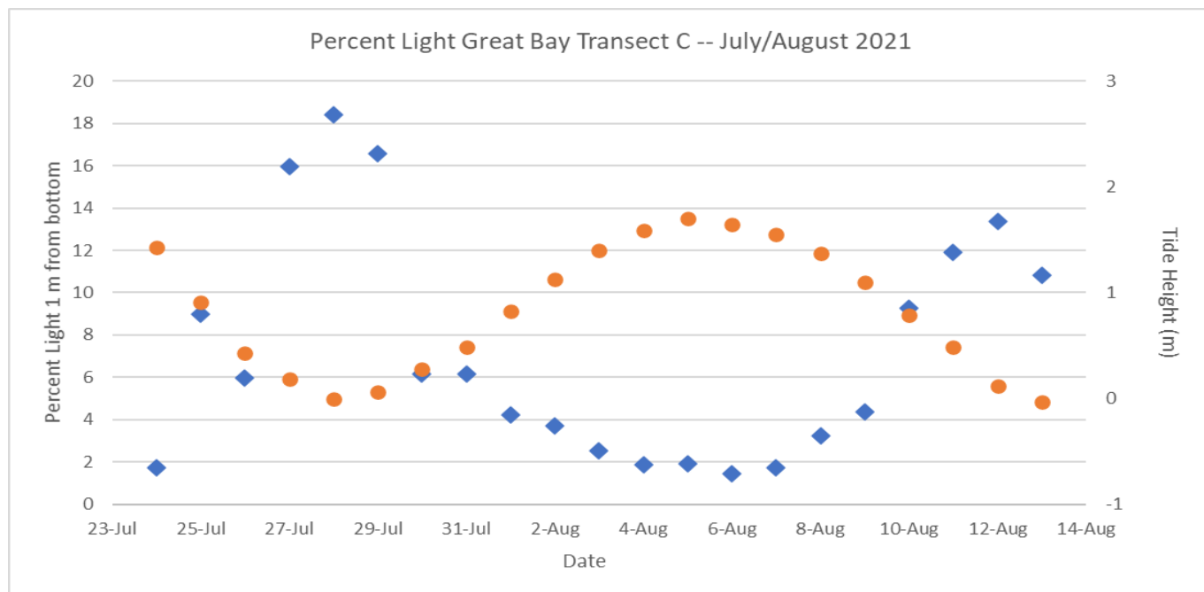
Figure 16. Mean values (blue diamonds) of percent light at 1 m from the bottom at Transect C, site NH9.2 (Great Bay), 7/24/2021 – 8/13/2021. Values represent means from data collected by HOBO sensors every 10 minutes,
