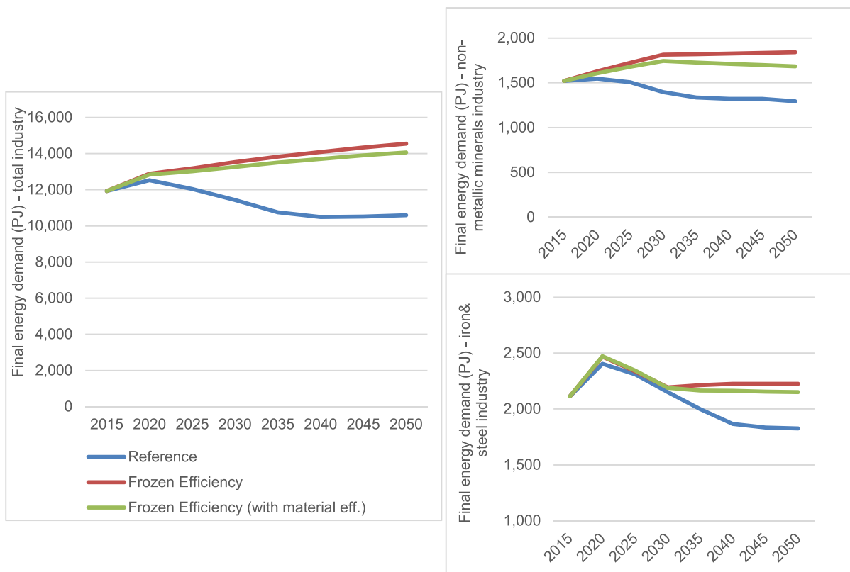
Fig. 4 Final energy demand in the EU27 + UK iron and steel and non-metallic minerals industry in the Reference and the Frozen Efficiency scenarios
