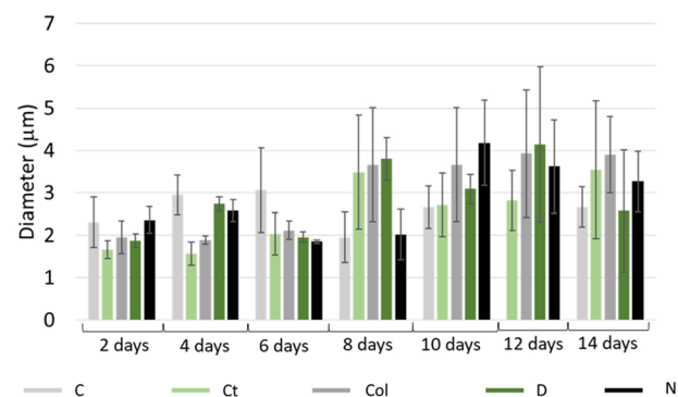
FIG. 3. Mean values and standard deviation of the different spider silk fiber diameters at different days. Overall, a slight increase in fiber diameter was observed, but among the groups on the same day, no significant differences were detected.
