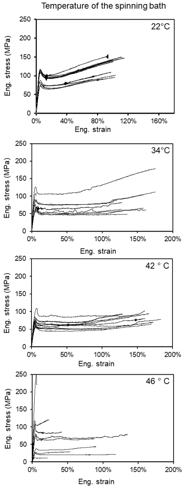
Supplementary Figure 18. Stress-strain curves of NT2RepCT fibers spun varying the temperature of the spinning buffer (22-46°C). At 22°C representative stress strain curves are shown. The calculated mechanical properties are shown in Figure 8 .
