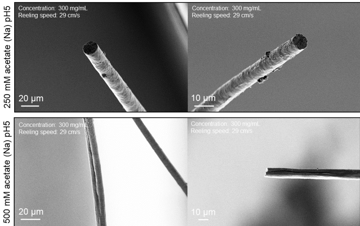
Supplementary Figure 16. Representative SEM images of NT2RepCT fibers spun using an acetate buffer (Na) with a concentration of 250 or 500 mM.
