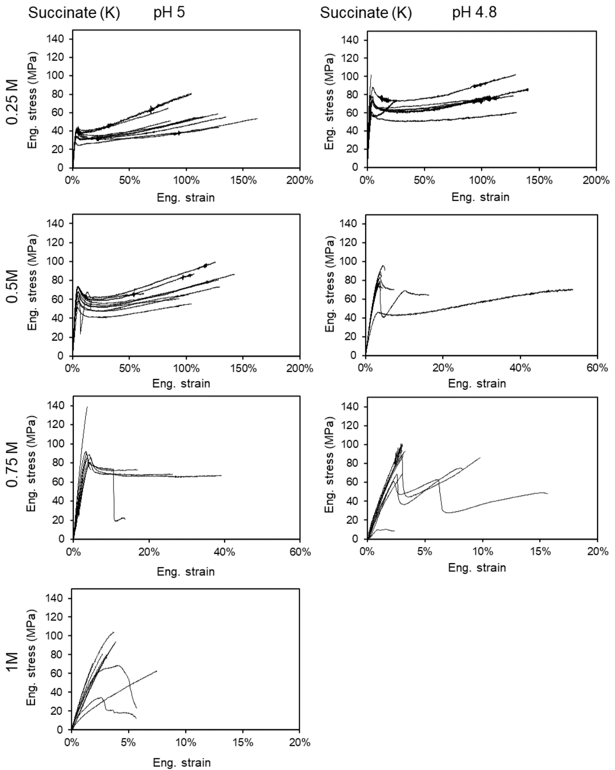
Supplementary Figure 10. Stress-strain curves of NT2RepCT fibers spun using different succinate buffers (pH 5 & 4.8 varied between 250 to 1M). The calculated mechanical properties are shown in Figure 4.
