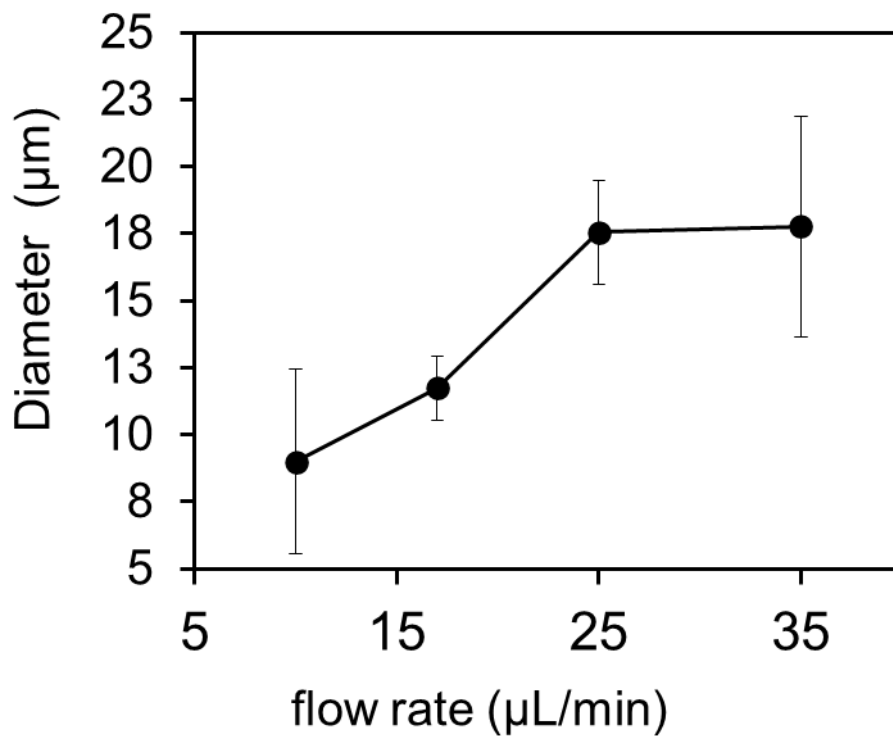
Supplementary Figure 3. Diameter of NT2RepCT fibers as a function of flow rate, using the same capillary size (86 μm).
