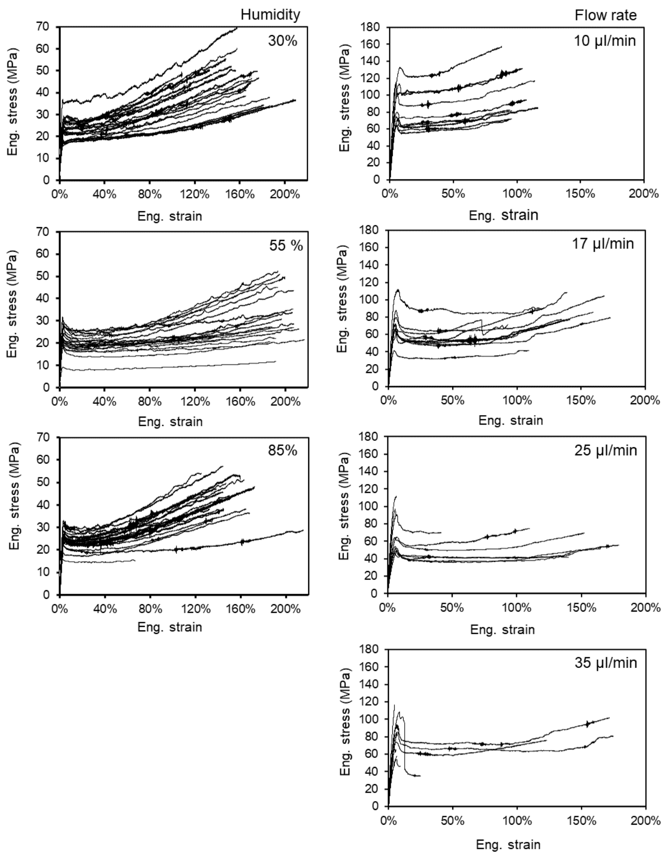
Supplementary Figure 5. Stress-strain curves of NT2RepCT fibers spun using different relative humidities and flow rates. The calculated mechanical properties are shown in Figure 3 .
