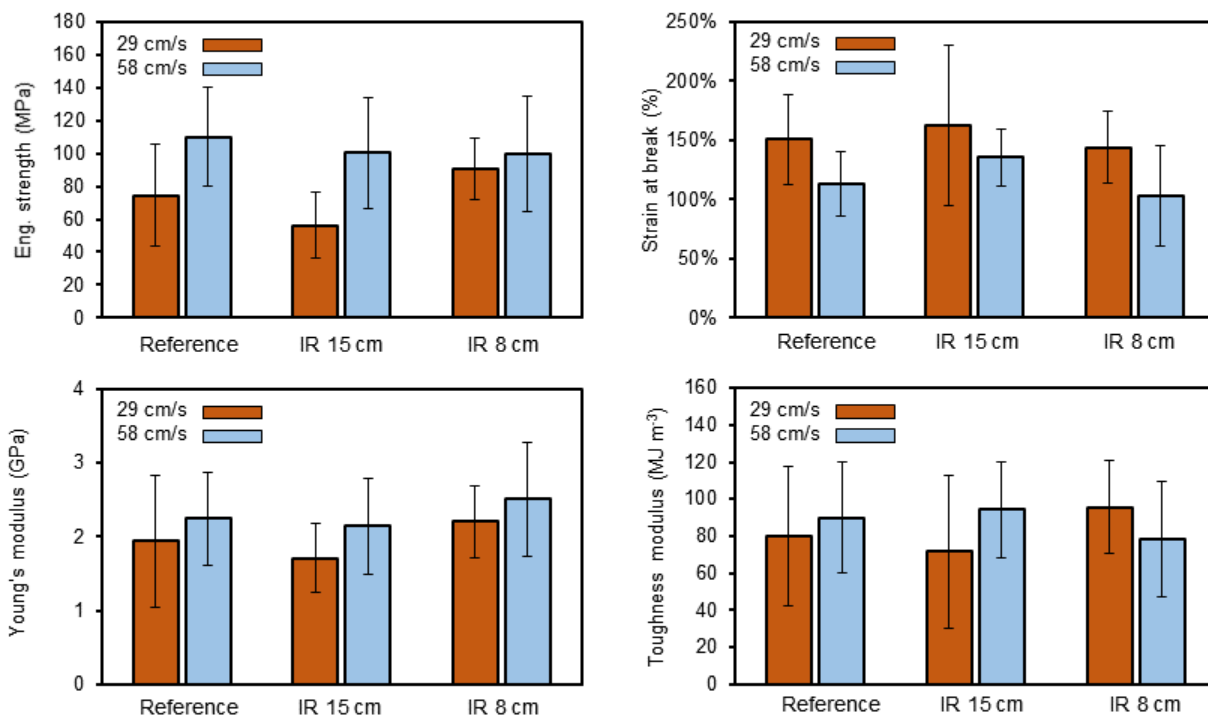
Supplementary Figure 19. Mechanical properties of NT2RepCT fibers under the influence of IR lamp placed in the vicinity of the collection wheel (distance: 8 cm or 15 cm). The reference fibers in this plot are the grand average of all fibers spun at 29 or 58 cm/s, as shown in Figure 6 . Other parameters relevant for this spinning experiment are found in Supplementary Table 2 .
