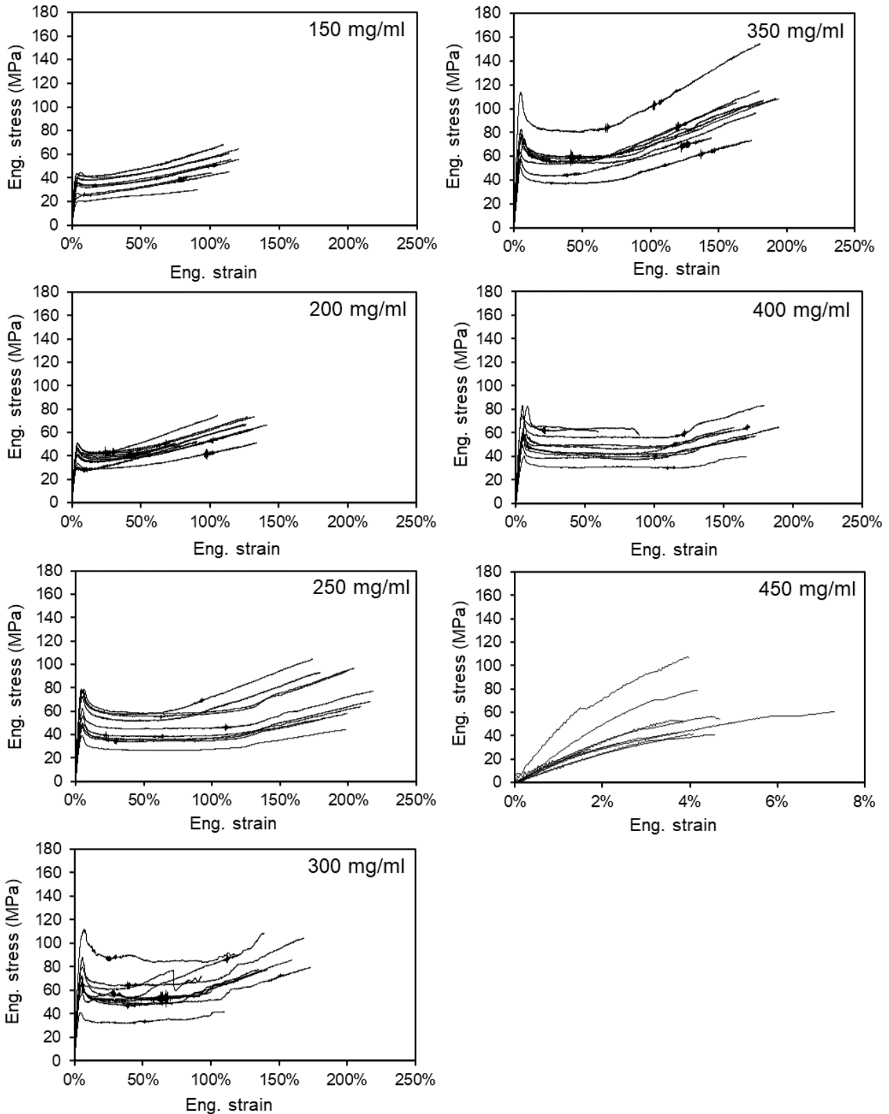
Supplementary Figure 4. Stress-strain curves of fibers spun using different NT2RepCT concentrations and using a 750 mM acetate (Na) spinning buffer with or without 150 mM NaCl. The calculated mechanical properties are shown in Figure 3 .
