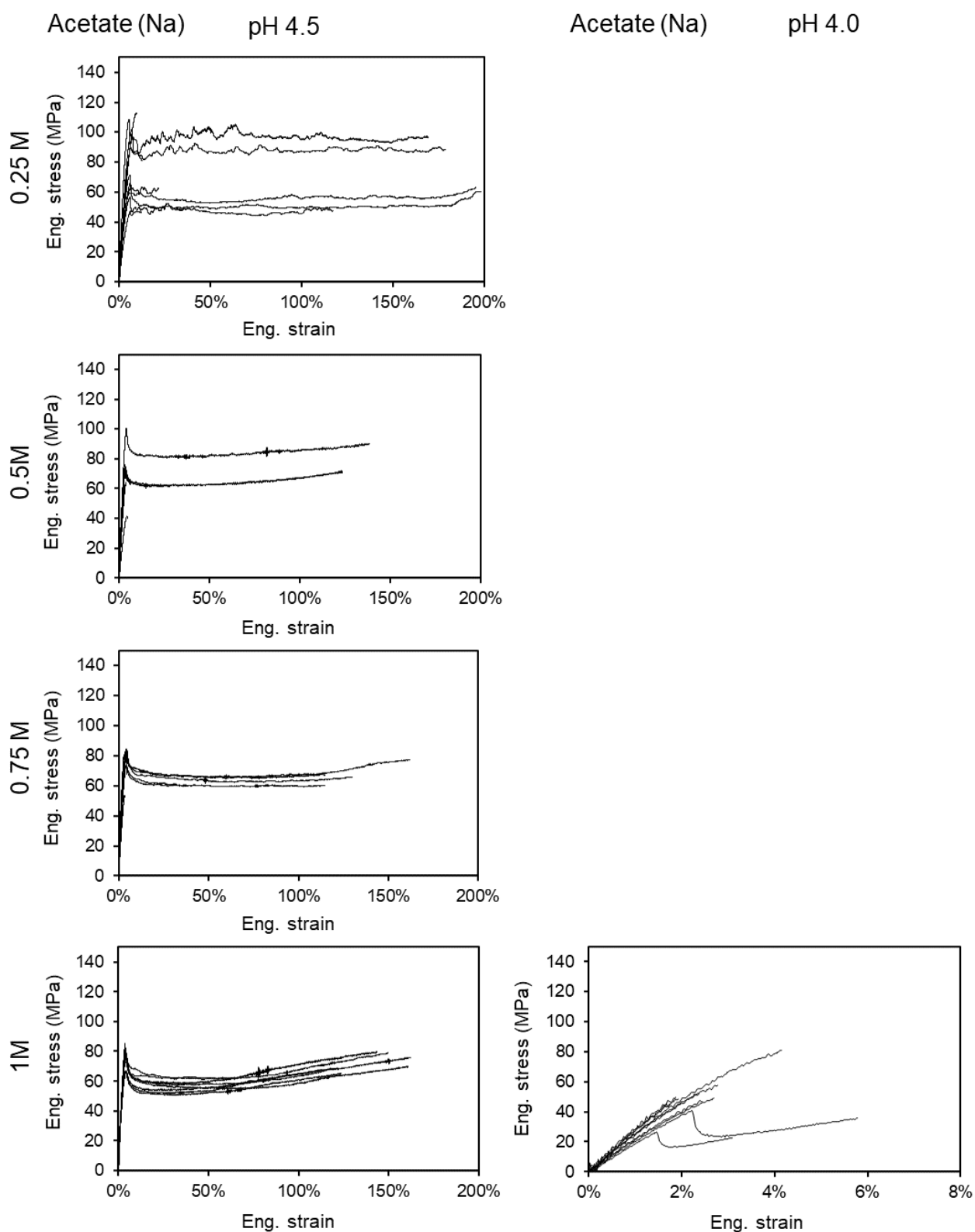
Supplementary Figure 9. Stress-strain curves of NT2RepCT fibers spun using different acetate buffers (pH 4.5 & 4.0 varied between 250 to 1M). The calculated mechanical properties are shown in Figure 4 .
