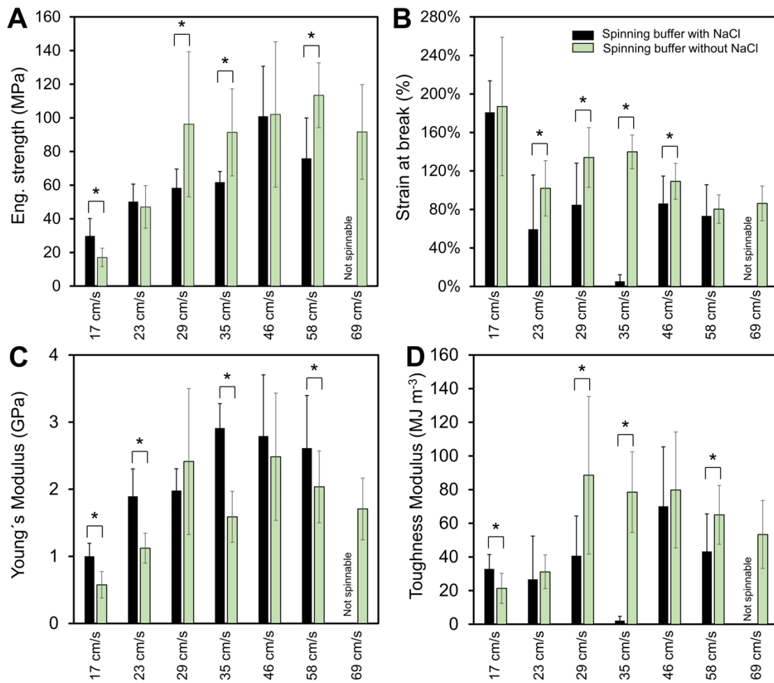
Supplementary Figure 14. Dependence of the mechanical properties of NT2RepCT fibers on the reeling speed, both with (black bars) and without 200 mM NaCl (light green bars) in the 750 mM acetate, pH 5, spinning buffer. The error bars indicate the standard deviation. At least 10 fibers were tensile tested for each reeling speed. A significant difference ( p < 0.05 ) is indicated with stars.
