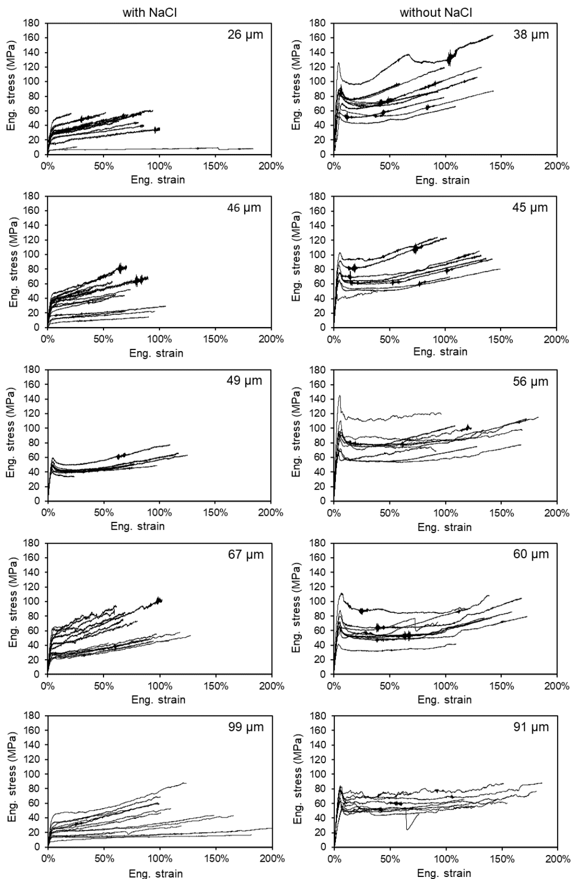
Supplementary Figure 1. Stress-strain curves of NT2RepCT fibers spun using different capillary diameters and using a 750 mM acetate (Na) spinning buffer with or without 150 mM NaCl. The calculated mechanical properties are shown in Figure 2 .
