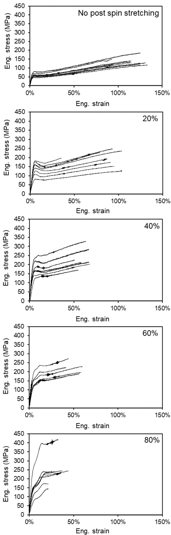
Supplementary Figure 20. Stress-strain curves of post-spin stretched NT2RepCT (0-80%). The calculated mechanical properties are shown in Figure 9 .
