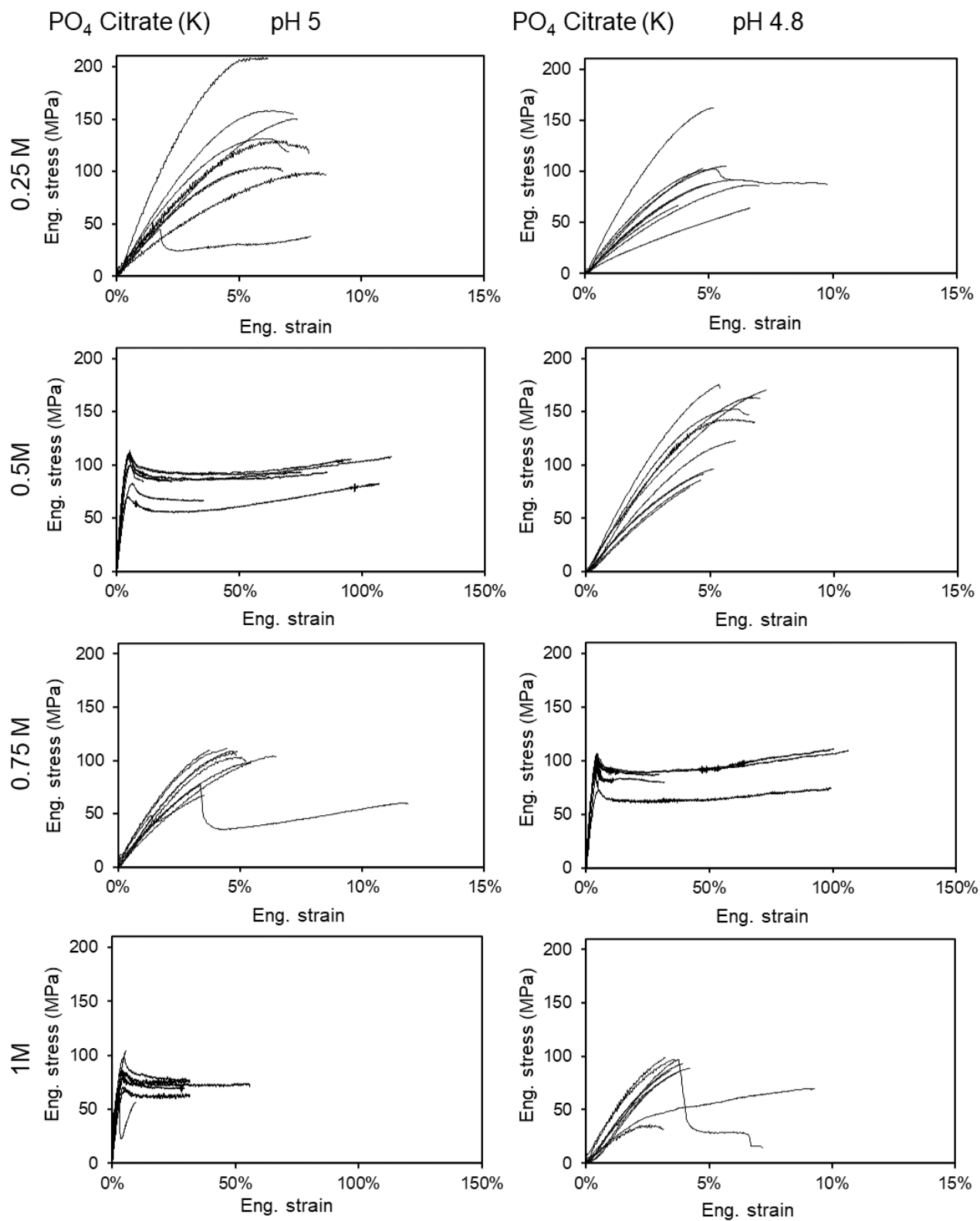
Supplementary Figure 12. Stress-strain curves of NT2RepCT fibers spun using different citrate-phosphate buffers (pH 5 & 4.8 varied between 250 to 1M). The calculated mechanical properties are shown in Figure 4 .
