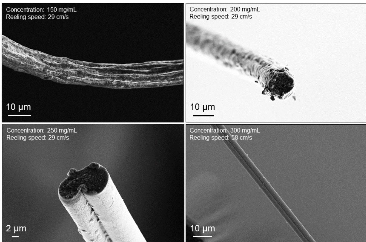
Supplementary Figure 17. Representative SEM images of NT2RepCT fibers spun using different protein concentrations in the spinning dope.
