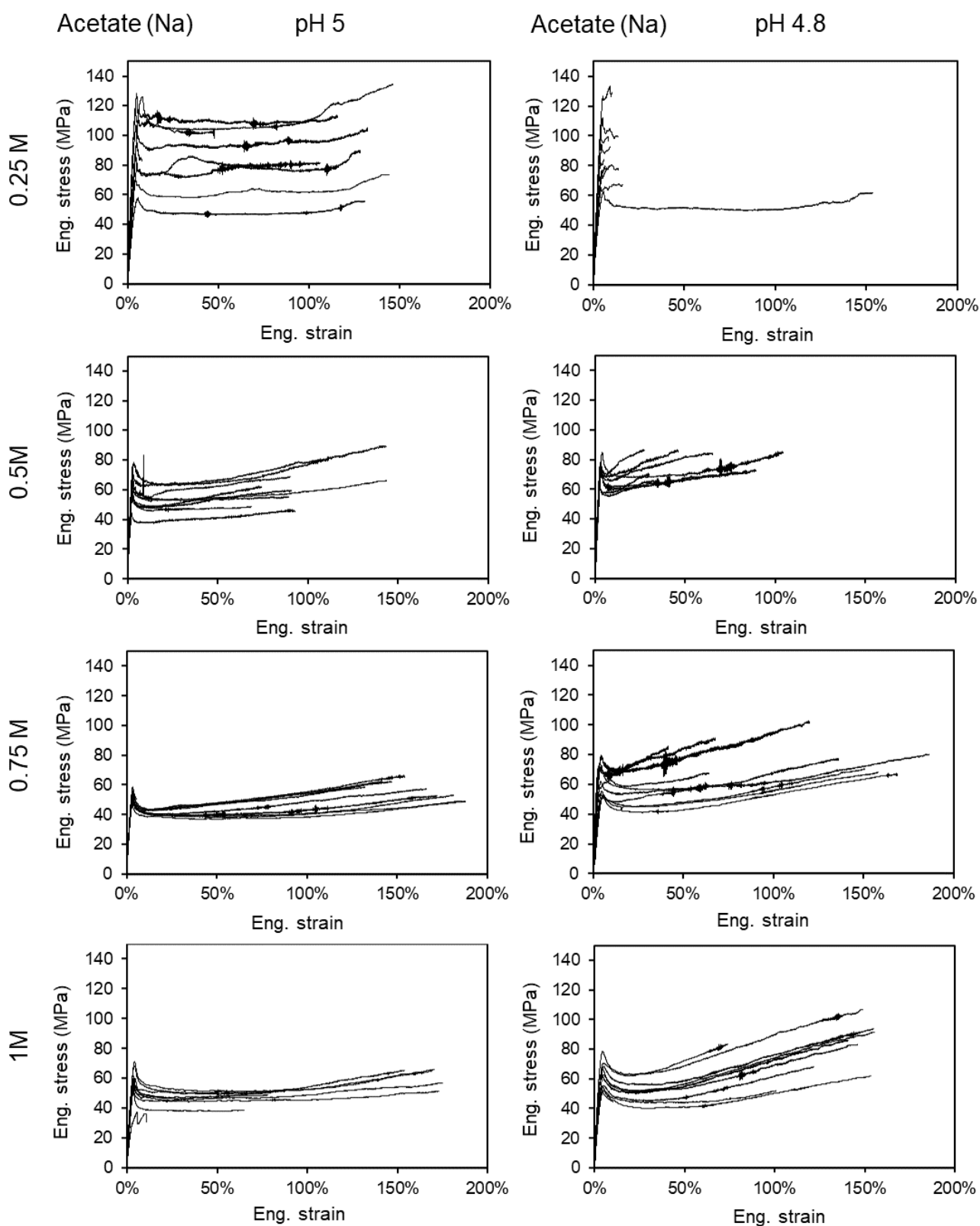
Supplementary Figure 8. Stress-strain curves of NT2RepCT fibers spun using different acetate buffers (pH 5 & 4.8 varied between 250 to 1M). The calculated mechanical properties are shown in Figure 4 .
