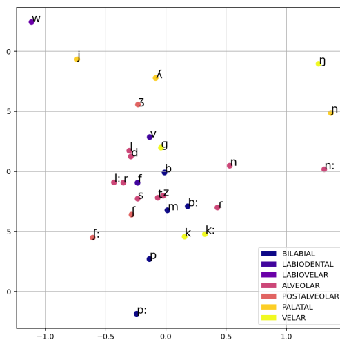
Figure 4: PCA of IT phonetic source embeddings (ES-IT RNN), coloured according to place of articulation.
