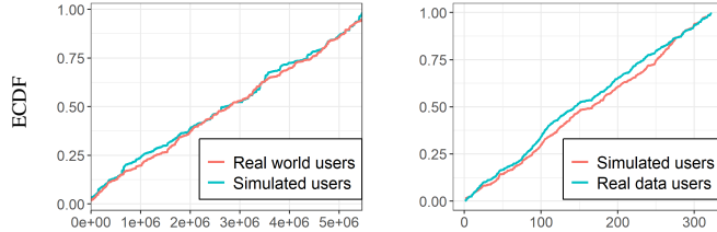
(a) Third-order probabilities (b) Nb of attributes per user Fig. 1: Comparison of ECDFs for actual platform users in \mathcal{D}_{\text{attributes}} and for the synthetic population generated.
