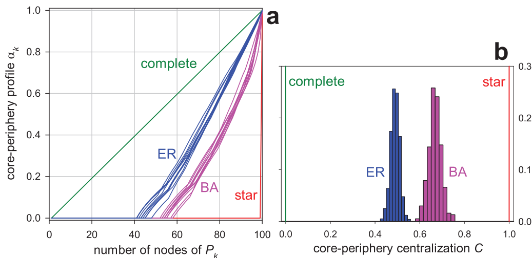
Figure 1 | Core-periphery profile and centralization of four types of artificial networks. (a). The core-periphery profile of the star network (the n - 1 peripheral nodes are connected to the center node only), of the complete (all-to-all) network, and of a few realizations of Erdős-Rényi ( ER ) and Barabási-Albert ( BA ) networks (10 realizations each, n = 100 , average degree \langle k \rangle = 4 ). (b). The histograms of the distribution of the cp-centralization C over 10^3 realizations of ER and BA networks ( n = 100 , \langle k \rangle = 4 ). The values of C for the complete and star networks are highlighted for comparison.
