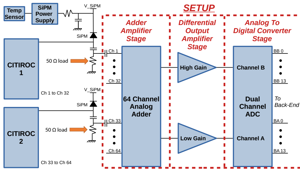
Figure 7. Scheme of the HG and LG channels. The signals from the 64-pixel SiPM array are added in a first stage (Adder Amplifier Stage), amplified and splitted in a high gain/low gain branch (Differential Output Amplifier Stage) and continuously digitized by a dual ADC (Analog To Digital Converter Stage). This circuitry represents a load of 50\ \Omega to the CITIROC inputs.
