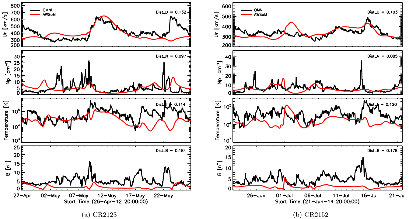
Figure 6. Data–model comparisons for CR2123 and CR2152 at 1 au. Panels (a) and (b) show the AWSoM results (in red) along the trajectory of the Earth and the solar wind plasma observations from the OMNI database (in black).
