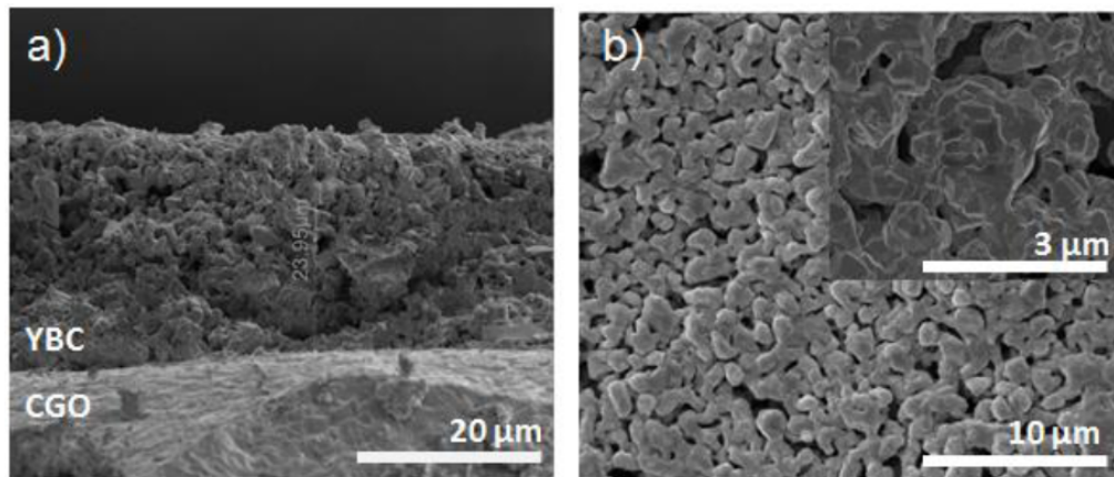
Figure 6: SEM images of a) the cross-section of YBC layer deposited on GDC and b) the top of the corresponding YBC electrode surface.
