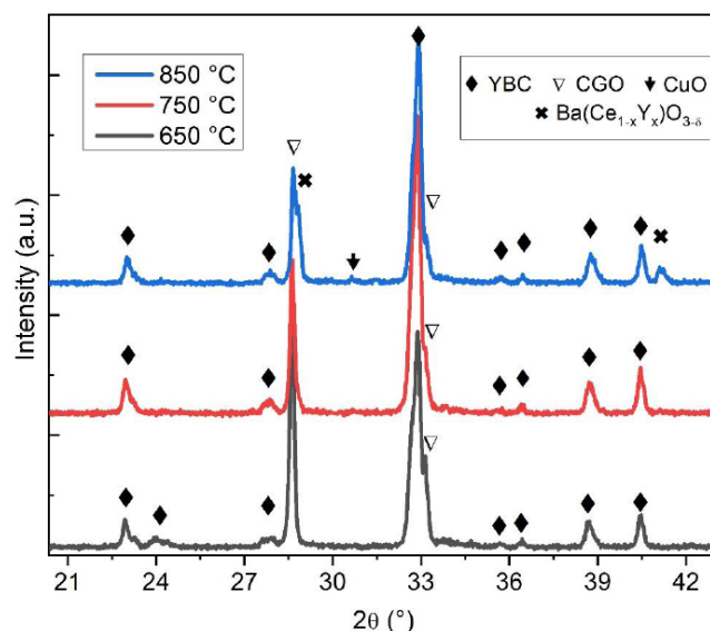
Figure 5: RT XRD patterns after reactivity tests between YBC and GDC powders in air.
