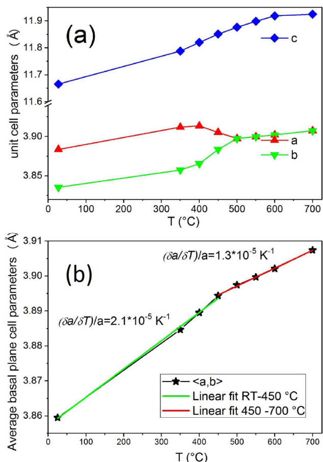
Figure 3: a) Evolution of lattice parameters as a function of temperature in air, where the phase transition occurs at \sim 425 °C. b) Fit of the evolution of \langle a,b \rangle parameters with temperature with associated coefficient of linear expansion.
