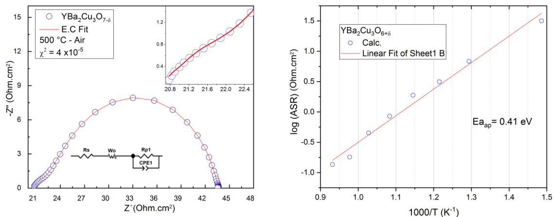
Figure 7: a) Fit of the impedance spectrum of YBC/GDC/YBC symmetrical cell measured at 500 \text{ }^\circ\text{C} in air; b) Arrhenius plot of ASR between 500 and 800 \text{ }^\circ\text{C} .
