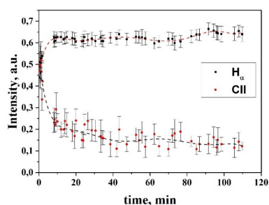
Fig. 5. Time evolution optical emission intensities of H_{\alpha} (656.2 nm) and C II (229.6 nm). ( U_a = 5 kV, p = 2.9 \times 10^{-2} Pa. Duty cycle: 10 ms (start), 40 ms (shutdown), one shot every 15 seconds.)
