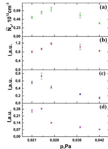
Fig. 4. Maximum average plasma density (a), optical emission intensities of H_\alpha , 656.2 nm (b); C II, 229.6 nm (c); O II, 441.5 nm (d); as a function of the initial gas pressure. ( U_a = 5.5 kV. Duty cycle: 10 ms (start), 20 ms (shutdown)).
