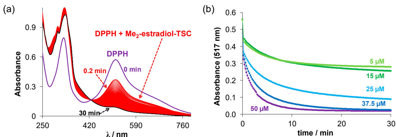
Figure 8. (a) Time-dependent changes of the UV–vis spectra of the DPPH• ( c = 50 \mu\text{M} ) in the presence of Me 2 -estradiol-TSC ( 50 \mu\text{M} ) in ethanol. ( T = 25 \text{ }^\circ\text{C} ); (b) absorbance changes of DPPH at 517 nm upon reaction with Me 2 -estradiol-TSC at different concentrations in ethanol plotted against time. ( c_{\text{DPPH}} = 50 \mu\text{M} ; c_{\text{ligand}} = 50, 37.5; 25; 15; 5 \mu\text{M} ; \ell = 1 \text{ cm} ; T = 25 \text{ }^\circ\text{C} ).
