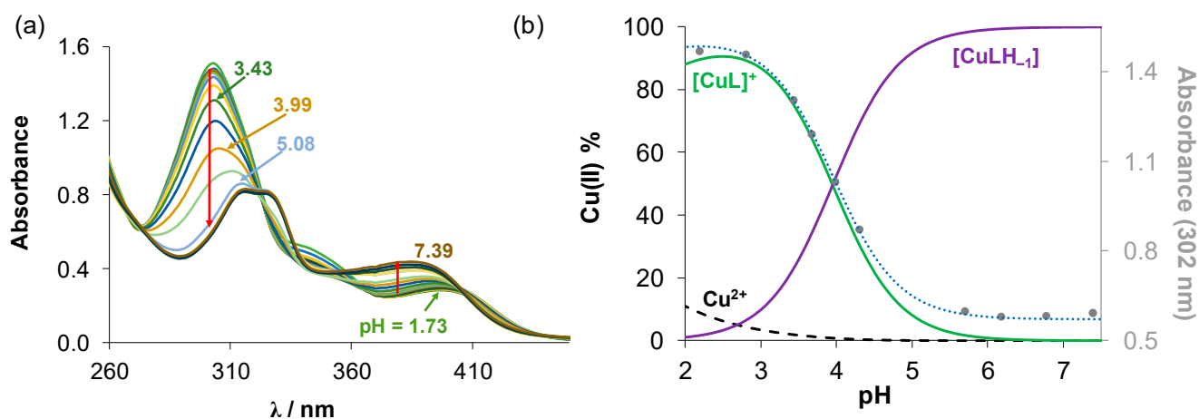
Figure 2. (a) UV-vis absorption spectra of the Cu(II)-estradiol-TSC (1:1) system in the pH range 1.73–7.39 in 30% ( v/v ) DMSO/H 2 O solvent mixture. (b) Concentration distribution curves calculated for the same system plotted together with the absorbance changes at 302 nm (●) with the fitted curve (dotted line). ( c_{\text{ligand}} = 20 \mu\text{M} ; c_{\text{Cu(II)}} = 20 \mu\text{M} ; T = 25.0 \text{ }^\circ\text{C} ; I = 0.1 \text{ M (KCl)} ).
