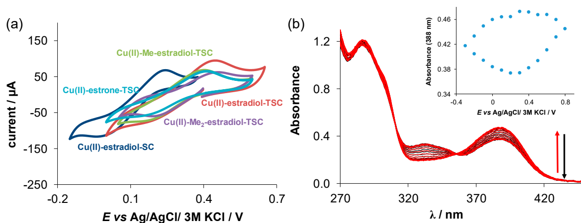
Figure 6. (a) Cyclic voltammograms of the Cu(II)-(T)SC (1:1) chemical systems in 90% ( v/v ) DMSO/H 2 O at 10 mV/s scan rate ( c_{\text{ligand}} = 1 \text{ mM} , c_{\text{Cu(II)}} = 1 \text{ mM} , pH = 7.40 (10 mM HEPES), T = 25 \text{ }^\circ\text{C} , I = 0.1 \text{ M} (nBu 4 NPF 6 )) E' vs. Ag/AgCl/3M KCl (V): Cu(II)-estradiol-SC = +0.10; Cu(II)-estrone-TSC = +0.28; Cu(II)-estradiol-TSC = +0.31; Cu(II)Me-estradiol-TSC = +0.29; Cu(II)-Me 2 -estradiol-TSC = +0.33; (b) UV-vis absorption spectra recorded for the Cu(II)-estradiol-SC system at the various potential values using the spectroelectrochemical cell. Inserted figure shows the absorbance values at 388 nm plotted against the potential. ( c_{\text{Cu(II)}} = 100 \text{ } \mu\text{M} ; l = 1 \text{ cm} ; I = 0.1 \text{ M} (NBu 4 PF 6 ); T = 25.0 \text{ }^\circ\text{C} , scan rate: 10 mV/s).
