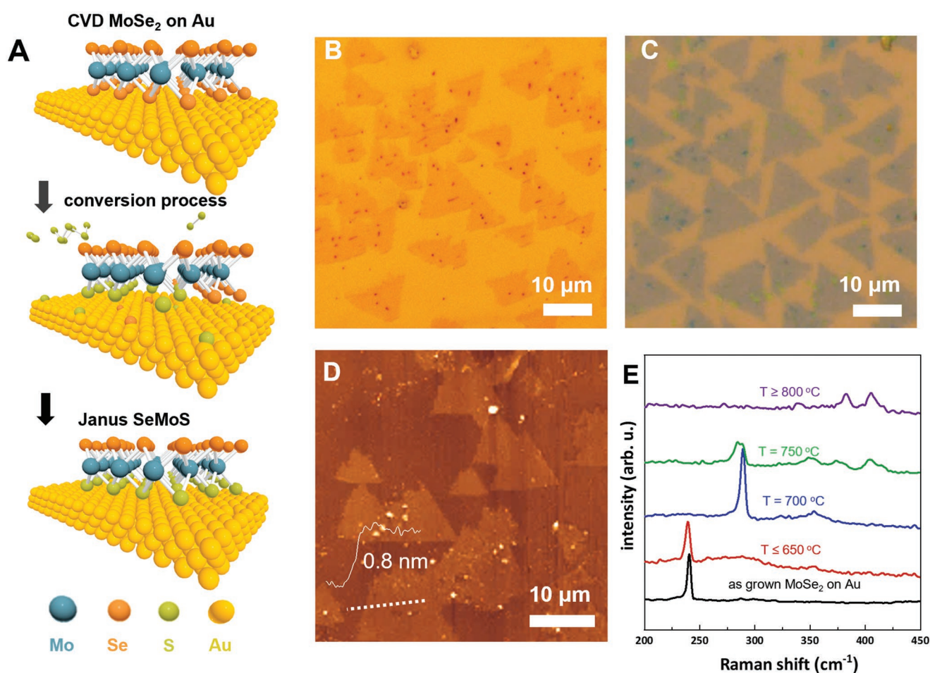
Figure 1. Synthesis and microscopic characterization of ML Janus SeMoS. A) Schematic illustration of the process for synthesizing ML Janus SeMoS. Initially, ML MoSe 2 is synthesized on Au foils by CVD, followed by a conversion process in which the MoSe 2 crystals were exposed to S vapor at 700 °C, replacing the bottom-layer Se atoms of MoSe 2 , which is in contact with the Au surface, by S atoms to form the ML Janus SeMoS. The Au surface absorbs and catalytically dissociates the S clusters. The dissociated S atoms are mobile on the Au surface at high temperature which migrates underneath the ML MoSe 2 and exchanges with the Se atoms in the bottom layer. On the other hand, replacement of the top Se layer is not energetically favorable as the S clusters elastically bounced back after colliding with the top Se layer, rather than dissociating and reacting. B,C) Optical microscopy images of ML Janus SeMoS, as grown on Au foil (B) and transferred on to SiO 2 /Si substrate (C). D) AFM topography image of transferred ML Janus SeMoS. The thickness of the ML Janus SeMoS is estimated as 0.8 \pm 0.2 nm from the height profile shown in the inset. E) Raman spectra recorded at room temperature using 532 nm excitation wavelength on pristine ML MoSe 2 and ML MoSe 2 exposed to S vapor at different temperatures. The optimum sulfurization temperature for obtaining Janus SeMoS is 700 °C.
