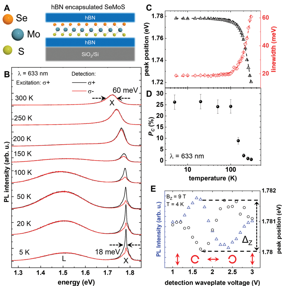
Figure 3. Temperature and valley polarization dependent optical properties of hBN-encapsulated ML SeMoS. A) Schematics of the encapsulated Janus SeMoS sample with hBN bottom and top layer. B) Temperature dependent photoluminescence (PL) spectra show the main excitonic emission (X) and up to 150 K also emission from localized states (L). For laser excitation polarization \sigma^+ both co-polarized (black) and counter-polarized (red) emission is plotted. C) From measurements as in (B), both the exciton transition linewidth (right axis, red symbols) and the transition energy (left axis, black symbols) are extracted and fitted, see text. D) The circular polarization degree P_c = (I_{\sigma^+} - I_{\sigma^-}) / (I_{\sigma^+} + I_{\sigma^-}) of the PL from (A) is plotted as a function of sample temperature. The error bars correspond to the standard deviation extracted over five different areas of the sample. E) PL measurements at T = 4\text{ K} in a magnetic field B_z = 9\text{ T} applied perpendicular to the sample surface. The detection polarization is varied by changing the voltage applied to a liquid crystal retarder, which yields the exciton Zeeman splitting \Delta_z . Excitation with linearly polarized light (equal intensity for both circular polarization states). The red arrows indicate the detection polarization state of the liquid crystal retarder for given voltages.
