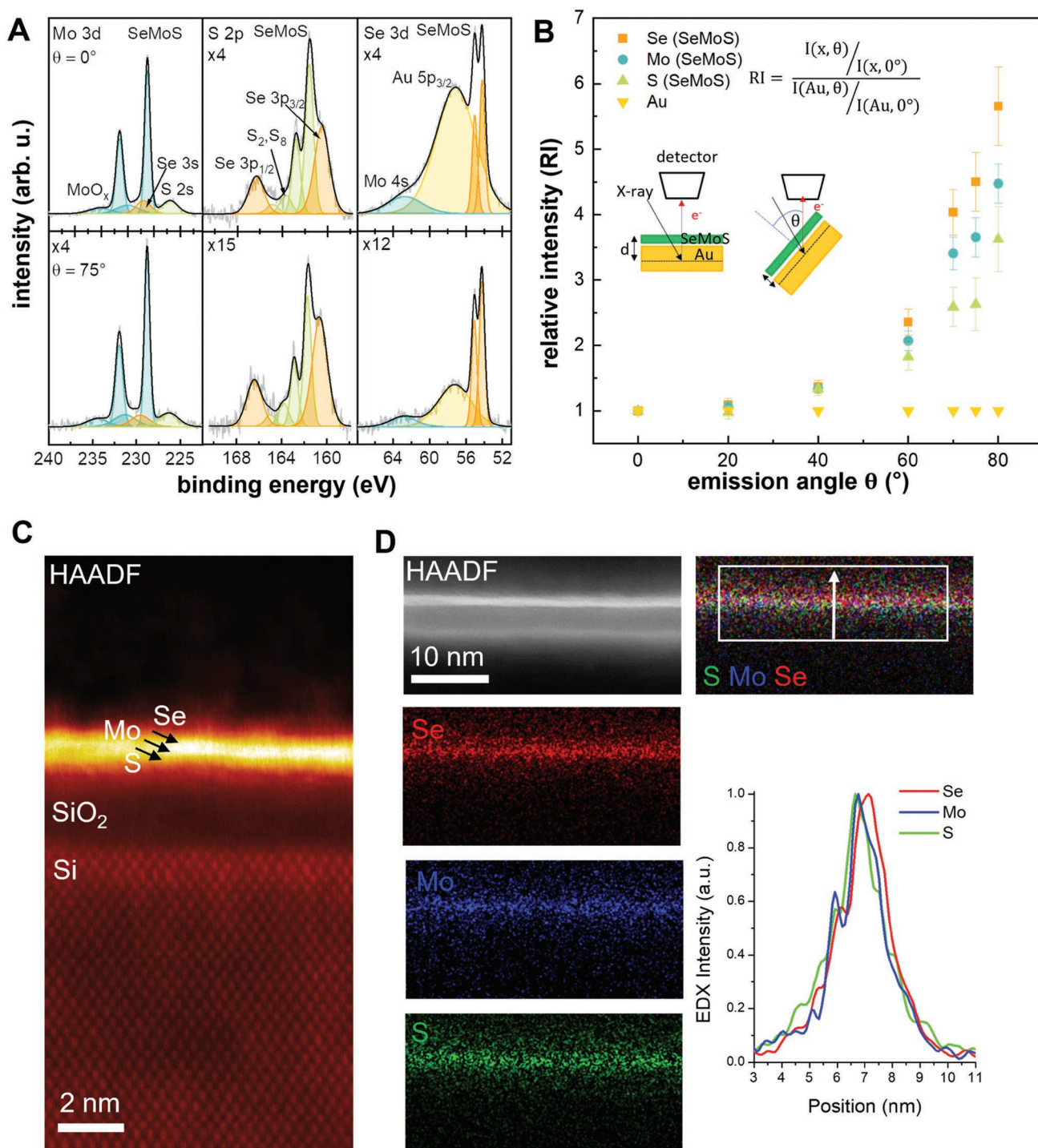
Figure 2. Angle-resolved XPS and TEM investigation of ML Janus SeMoS. A) High-resolution Mo 3d, S 2p, and Se 3d XP spectra of as-grown ML Janus SeMoS on Au foil measured at an emission angle ( \theta ) of 0^\circ (normal emission, top) and 75^\circ (bottom), respectively. The fitted components have been named in the figures and discussed in detail in Note S7, Supporting Information. For better representation, the intensities of the spectra were multiplied by the factors represented in the respective figures. B) Relative intensities (RIs) of the Janus SeMoS components represented by Mo 3d, S 2p, and Se 3d peaks as well as the substrate reference Au 4f peak calculated according to the formula written in the inset are plotted for certain emission angles. Thereby, I(x, \theta) , I(x, 0^\circ) , I(Au, \theta) , and I(Au, 0^\circ) are the intensities of each element ( x = \text{Se, Mo, S, Au} ) at \theta and at normal emission as well as the intensities of Au at \theta and at normal emission. In addition in the inset, two schemes are shown to illustrate the set-up for ARXPS ( \theta = 0^\circ and 60^\circ ), whereby d is the information depth. C) Atomically resolved cross-sectional HAADF-STEM (Z-contrast) image of the interface of Janus structure on SiO 2 /Si substrate. Two bright layers (Se and Mo) above a third layer (S) are visible on top of the native SiO 2 layer and the crystalline Si. The arrows mark the three different layers. D) EDX elemental maps of S, Se, and Mo together with the corresponding HAADF reference image showing three layers. The composed RGB colormap and the integrated linescan of the EDX intensity shows the ordering structure of the Janus from bottom interface to the top surface as S/Mo/Se.
