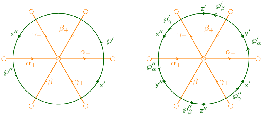
Fig. 18 Left: Let x', x'' be the two preimages of x on \Sigma as shown. Right: Let y', y'', z', z'' be the lifts of y, z as shown, \wp' = \wp'_\gamma \wp'_\beta \wp'_\alpha and \wp'' = \wp''_\gamma \wp''_\beta \wp''_\alpha
