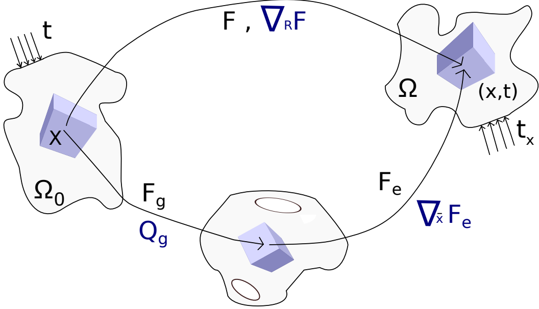
Figure 1: Illustration of the material isomorphism involving the first-order transplant \mathbf{F}_g and the second-order transplant \mathbf{Q}_g in the intermediate grown state.
