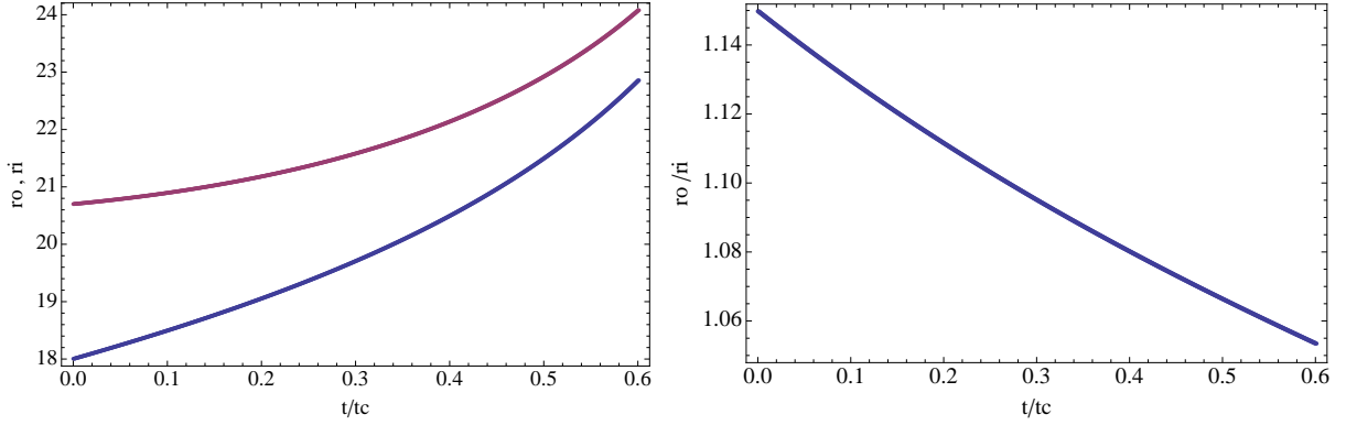
Figure 3: Evolution of the outer and inner radii (left) and thickness ratio (right) according to the evolution equation in Eq.(128) for an ascending aorta (length-scales given in mm). The numerical solution has been calculated setting p_i=160\text{mmHg} , c_1=150\text{KPa} and J(0)=1 , with an initial homogeneous deformation ( g_\theta=0.777 ). The depicted curves have been obtained solving Eq.(115) using Newton's method.
