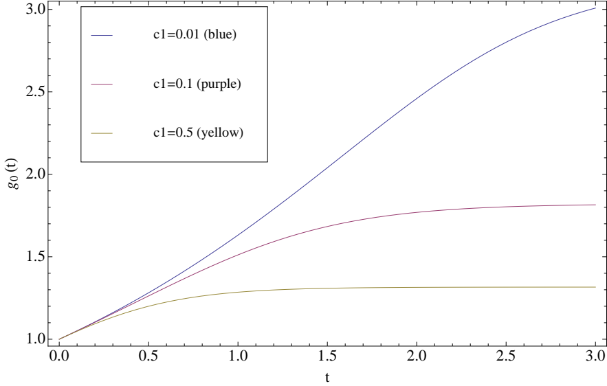
Figure 2: Plot of the homogeneous growth function g_0(t) over time t , from Eq.(94), shown for several values of elastic coefficient c_1 (all the other material coefficients are set equal to one).
