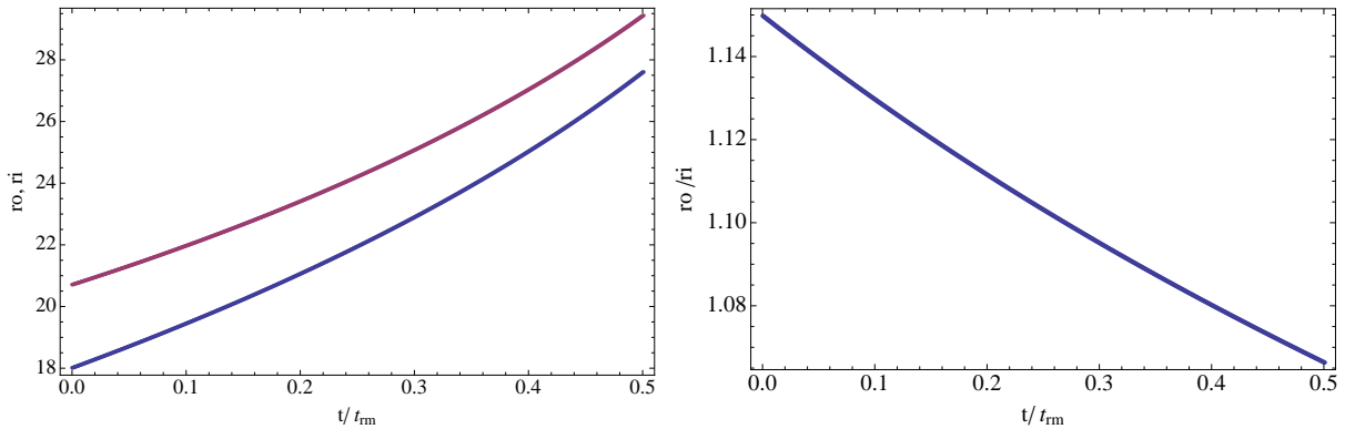
Figure 4: Evolution of the outer and inner radii (left) and thickness ratio (right) according to the evolution equation \dot{g}_\theta/g_\theta = -2\dot{g}_r/g_r = 1/t_{rm} for an ascending aorta (length-scales given in mm). The numerical solution has been calculate setting p_i=160\text{mmHg} , c_1=150\text{KPa} and J(0)=1 , from an initial homogeneous deformation ( g_\theta=0.777 ). The depicted curves have been obtained solving Eq.(115) using Newton's method.
