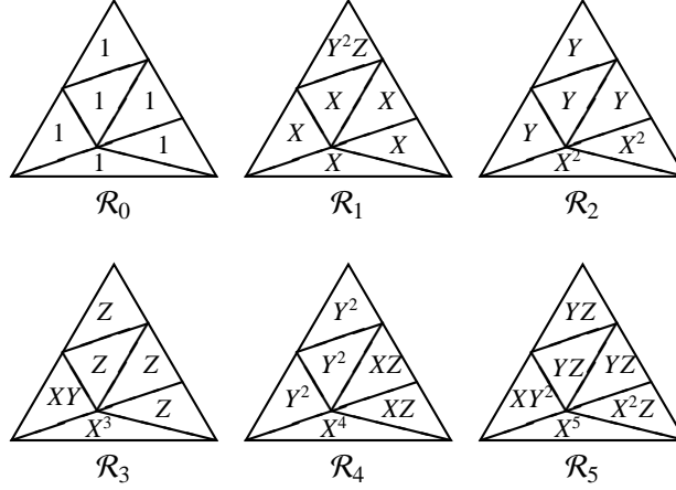
Figure 9. Monomial generators of \mathcal{R}_i for \mathbb{Z}_6 -Hilb( \mathbb{C}^3 )
