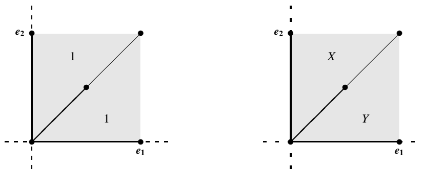
Figure 8. Monomial generators of \mathcal{R}_0 and \mathcal{R}_1 for \mathbb{Z}_2 -Hilb( \mathbb{C}^2 )
