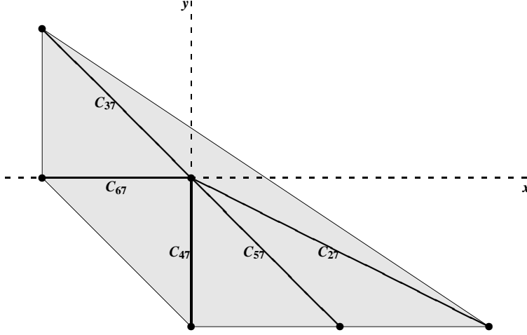
Figure 6. Fan for D_7 ( Star(\rho_7) )
