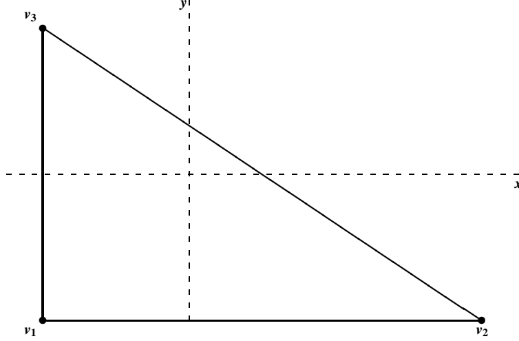
Figure 1. \mathbb{C}_6^3 fan
