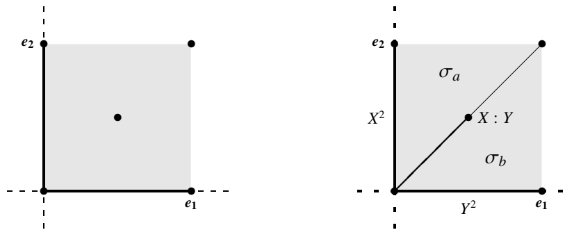
Figure 3. Fan for C^2/\mathbb{Z}_2 and \mathbb{Z}_2 -Hilb( C^2 ) in L = \mathbb{Z}^2 + \frac{1}{2}(1, 1)
