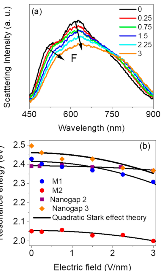
Figure 5. (a) Measured dark-field scattering spectra as a function of applied electric field. (b) Scattering peak position as a function of applied electric field for modes M1 and M2, alongside the scattering peak energies for two additional nanogaps. Solid curves are quadratic fits according to Stark shift dependence in conjugated polymers E(F) = E_0 - \frac{1}{2}\alpha F^2 .
