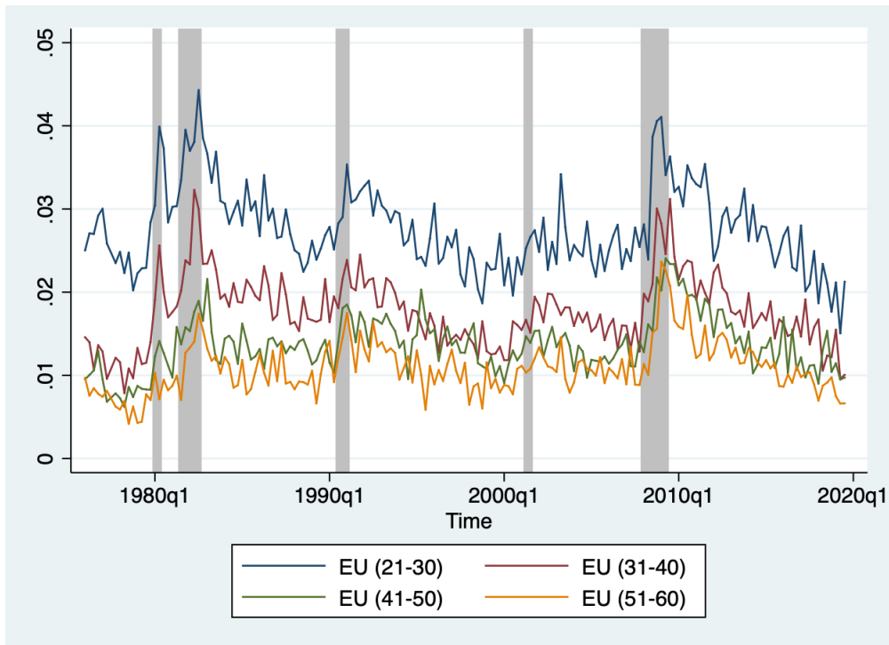
(b) u , v and tightness
