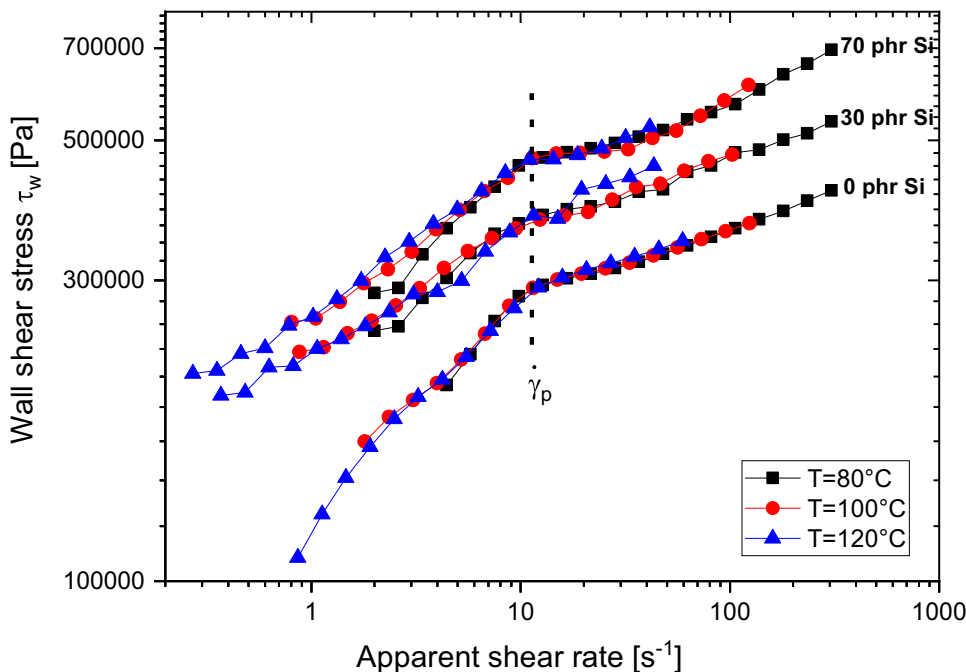
Fig. 14 Master flow curves for the different compounds
