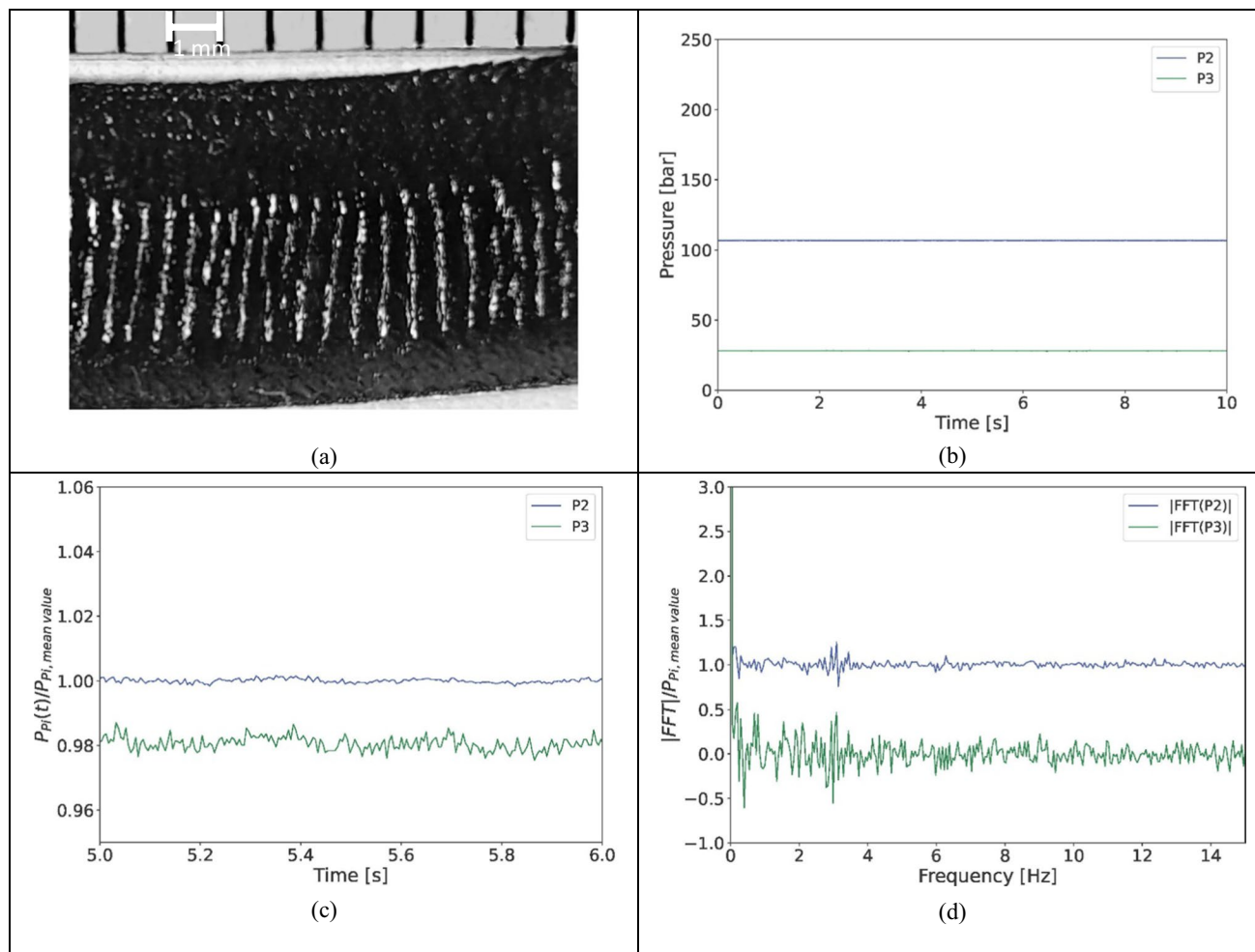
Fig. 6 Unfilled SBR extruded at a shear rate of \dot{\gamma}_{\text{app}} = 33\text{ s}^{-1} . a Image (total length of 1 cm). b Pressure vs time over 10 s. c Zoom in for relative pressure vs time over 1 s (normalized and shifted vertically). d Relative FFT spectrum (normalized and shifted vertically)
