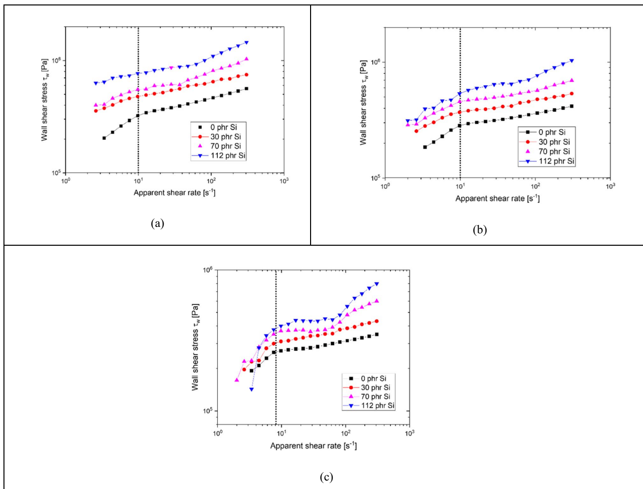
Fig. 3 Flow curves from a capillary rheometer for SBR compounds with 0 phr, 30 phr, 70 phr, and 112 phr silica at T = 80 \text{ °C} and L/D ratios of a L/D = 5/1 , b L/D = 10/1 , and c L/D = 20/1
