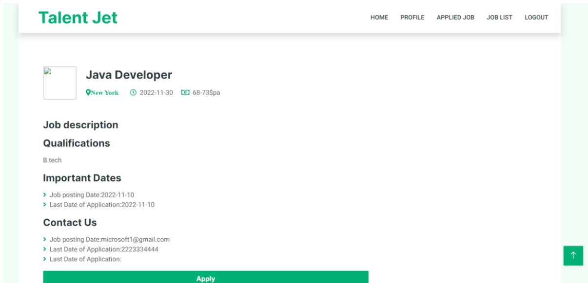
Figure 12: Job Detail
