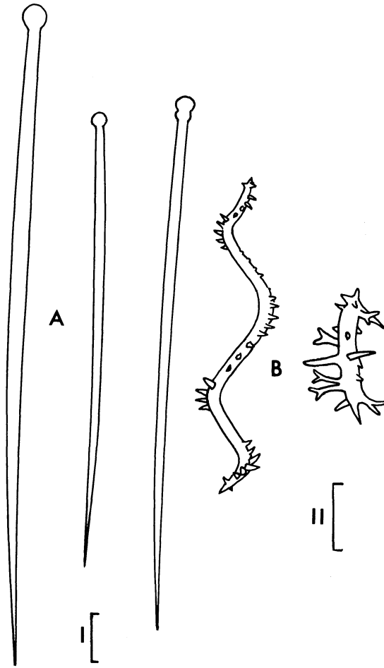
Fig. 12. Spicules of Cliona aprica n. sp. forma aprica . A. Tylostyles. B. Spirasters. Scale I (A) = 25 \mu\text{m} ; scale II (B) = 5 \mu\text{m} .
