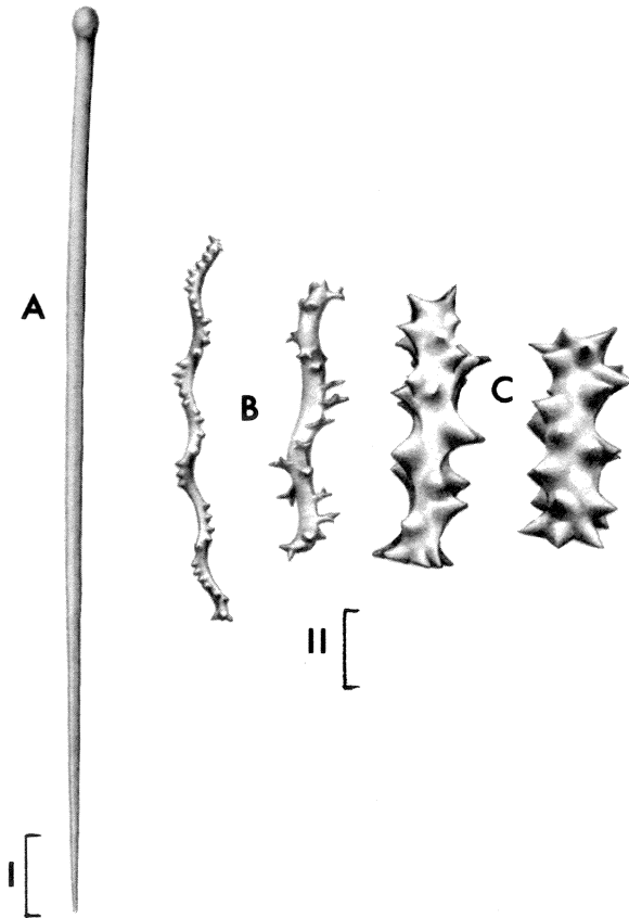
Fig. 1. Spicules of Cliona schmidti (Ridley). A. Tylostyle. B. Thin spirasters. C. Stout spirasters. Scale I (A) = 25 \mu\text{m} ; scale II (B,C) = 10 \mu\text{m} .
