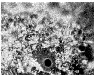
Fig. 17. Oscule of Cliona lampa de Laubenfels inhabiting dead coral. Scale = 2 mm. Fig. 18. Excavations of Cliona lampa inhabiting dead coral. Scale = 5 mm. Fig. 19. Excavations of Cliona vermifera Hancock. Scale = 3 mm. Fig. 20. Ostial and oscular (lowermost edge) papillae of Cliona vermifera Hancock. Scale = 3 mm. Fig. 21. Oscule of Cliona aprica n. sp. forma aprica inhabiting dead coral. Scale = 3 mm.
