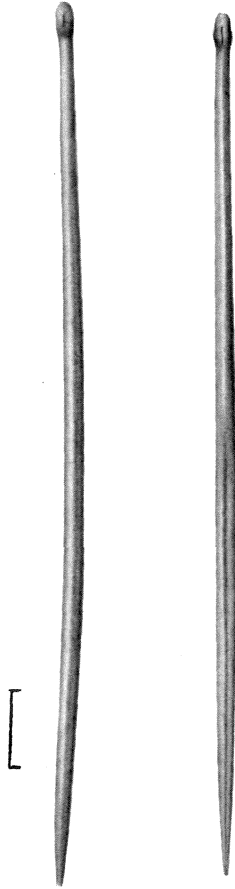
Fig. 7. Tylostyles of Cliona delirix n. sp. Scale = 25 \mu\text{m} .
