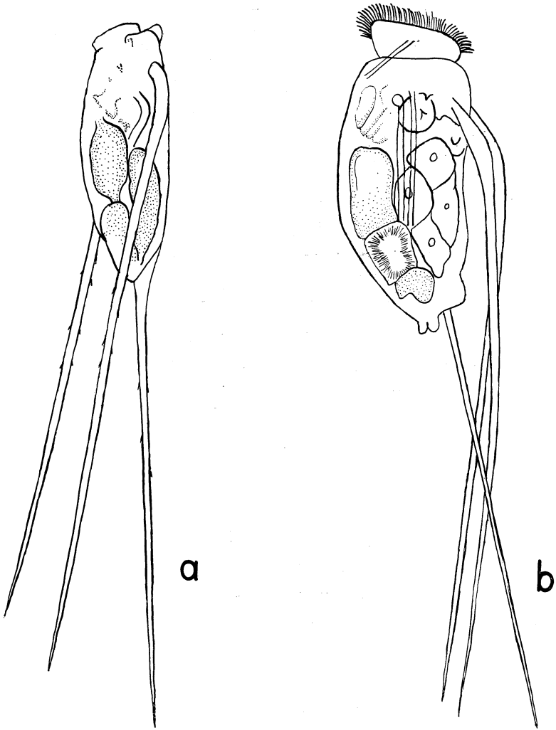
Figure 1a. Filinia pejlery sp. n. Ootacamund, Nilghiri Hills, S. India (holotype), \times 230 . Figure 1b. F. terminalis (Plate), first figured specimen, Dundee, Scotland; after Calman (1892).
