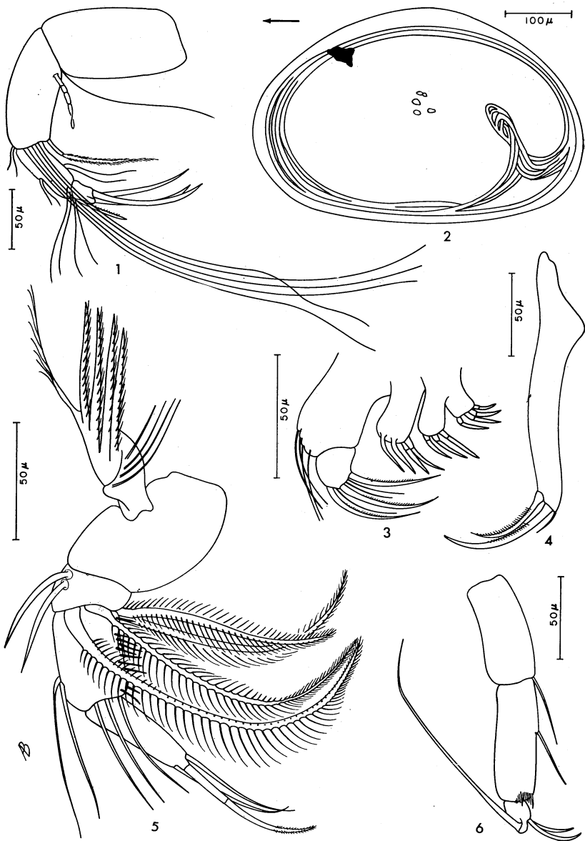
Cyprid petenensis n. sp.—Drawings of figures 1, 3, 4, 5, and 6 were made from the female holotype stained with lignin pink and mounted in polyvinyl lactophenol. The drawing of figure 2 was made from the androtype stained in a 1% alcoholic solution of eosin Y and mounted in Canada balsam. 1. Second antenna of female holotype. 2. Lateral view of right valve of androtype. 3. Maxilla and maxillary palp of female holotype. 4. Furcal ramus of female holotype. 5. Mandibular palp of female holotype. 6. Third thoracic appendage of female holotype.
