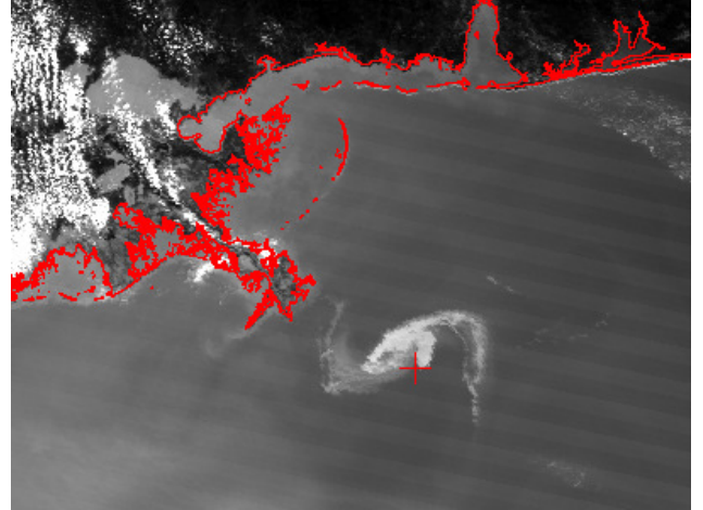
Figure 2: April 29, 2010 - MODIS day-time grayscale composition image of FEI. The red cross indicates the oil platform coordinates; the red line indicates the coastline.
