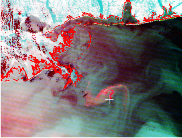
Figure 3: April 29, 2010 - MODIS day-time IR false color composition image. The white cross indicates the oil platform coordinates; the red line indicates the coastline.
