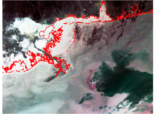
Figure 5: May 05, 2010 - MODIS night-time IR false color composition image. The white cross indicates the oil platform coordinates; the red line indicates the coastline.
