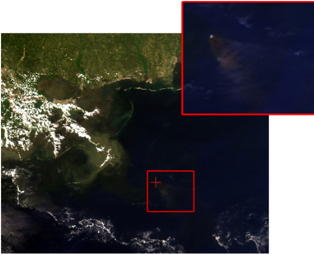
Figure 1: April 21, 2010 - MODIS true color composition image of the study area. The red cross indicates the oil platform coordinates; the red box indicates the zoom area on the platform fire and smoke plume.
