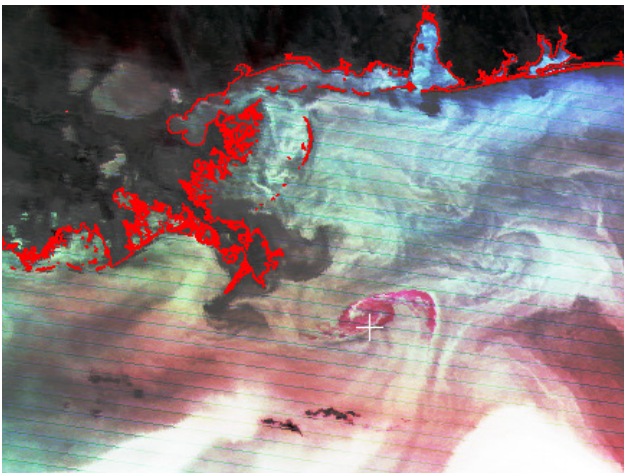
Figure 4: April 29, 2010 - MODIS night-time IR false color composition image. The white cross indicates the oil platform coordinates; the red line indicates the coastline.
