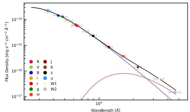
Figure 6. SED fit of AT 2016jbu at –11 days before Event B maximum. Extinction-corrected photometry is grouped into 1-day bins and weight-averaged. Flux errors are given as standard deviation of bins. Horizontal error bars represent the approximate filter band-pass. The hot blackbody is given in blue, the cooler blackbody in red, and the black line is a compound model. We note a similarity with the SED for SN 2009ip presented in Margutti et al. (2014).
