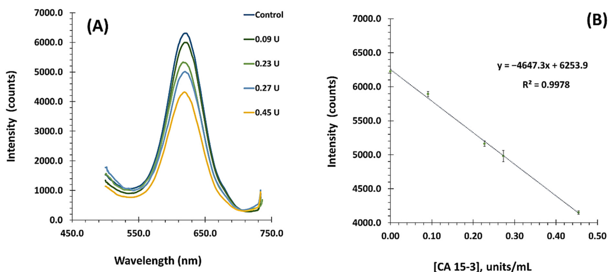
Figure 6. (A) Emission spectra of QD conjugates during protein recognition. (B) The calibration curve was performed in 10-fold diluted commercial human serum. The analysis was conducted using a photomultiplier tube voltage of 410 PMT and an excitation wavelength of 380 nm ( n = 3 ).
