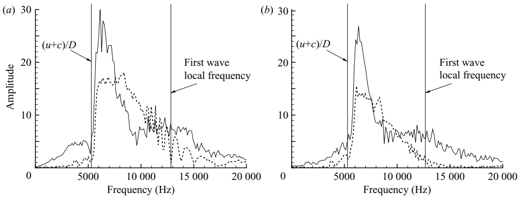
FIGURE 12. (a) Fourier transform of total pressure signal at measurement station x = 0.97 m ( x/D = 12 ): experimental (—) and numerical ( \cdots ) results for d = 56 mm ( d/D = 0.7 ) in the (ideally constant) post-shock region. The limiting frequencies f_\infty = (u + c)/D and the local frequency of the first wave are also indicated. (b) Fourier transform of total pressure signal at measurement station x = 1.65 m ( x/D = 20 ).
