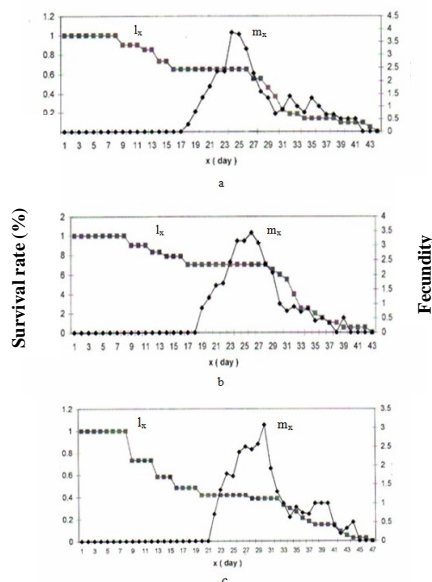
Figure 1. The age specific survival ( l_x ) and fecundity ( m_x ) of T. tabaci populations on onion (a, Golestan; b, Khorasan Razavi) and tobacco (c, Mazandaran), at 25°C, 50% RH and 16: 8 h L: D.
