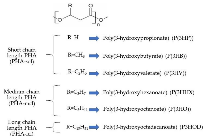
Figure 3. Chemical structure of PHAs and their classification based on the associated R-group, reproduced from [17,22].
