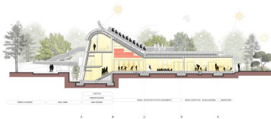
Figure 3: Cross section
