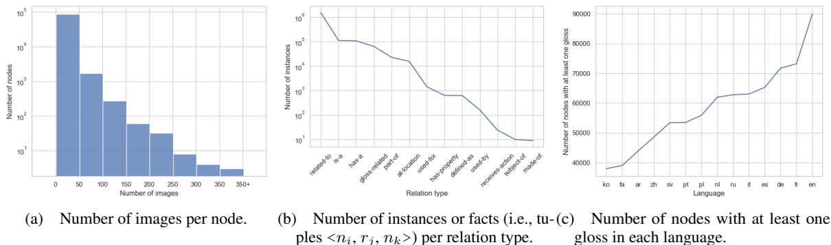
Figure 2: VisualSem data statistics.
