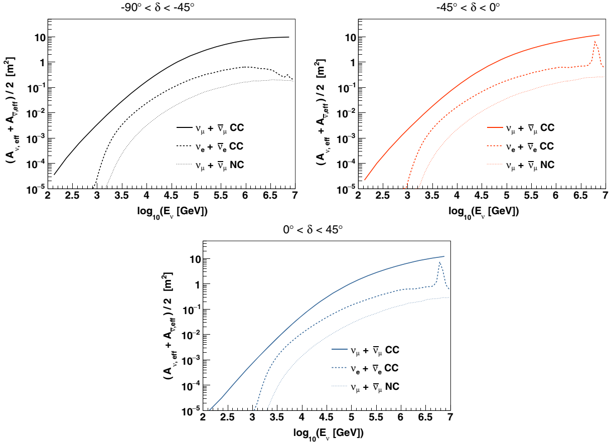
FIG. 1. Effective area for \nu_{\mu} + \bar{\nu}_{\mu} CC events after the track selection cuts (solid line) and for \nu_e + \bar{\nu}_e CC and \nu_{\mu} + \bar{\nu}_{\mu} NC events after the shower selection cuts (dashed lines) considering three declination ranges.
